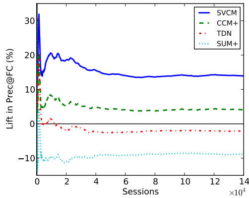
Figure 1: Prec@1 (left) and Prec@FC (right) of various user models relative to the deployed model. SVCM is the Sequential View Click Model, TDN is the model in [9], SUM is the Session Utility Model of [7], CCM is the Cascade Click Model of [6]. All models were trained using SGD (See Figure 3).
