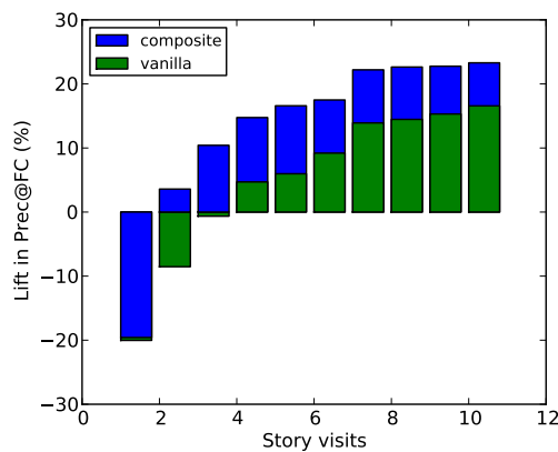
Figure 4: Lift in Prec@FC achieved by SVCM over deployed system vs number of user visits (right) and vs the number of times a story was displayed (left).
