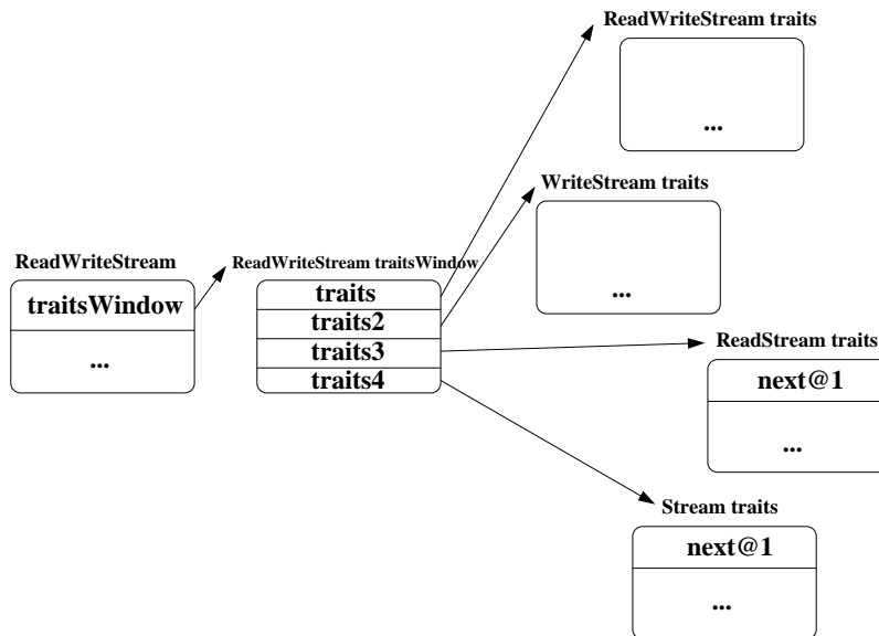
Fig. 11. Slate’s new traits inheritance model allows the more desirable breadth-first sequencing of methods.
