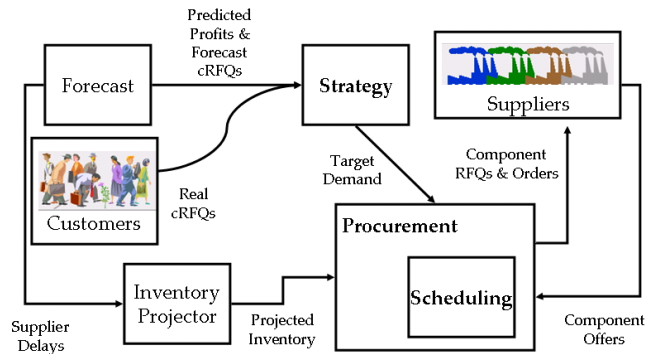
(b) B2B Interaction Overview
