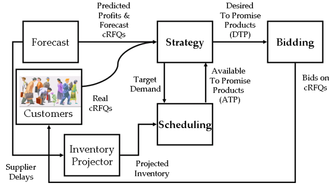
(a) B2C Interaction Overview
