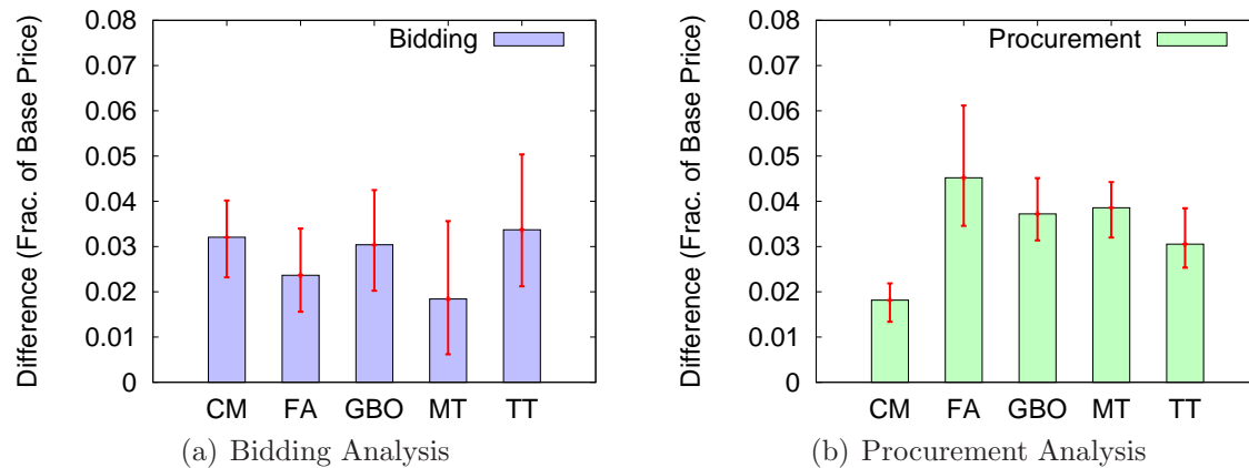
Figure 15: The mean (with 95% confidence intervals) difference between each of the top 5 agents’ average game unit price and the best unit price in the game, during the second week of the 2005 TAC SCM seeding rounds.
