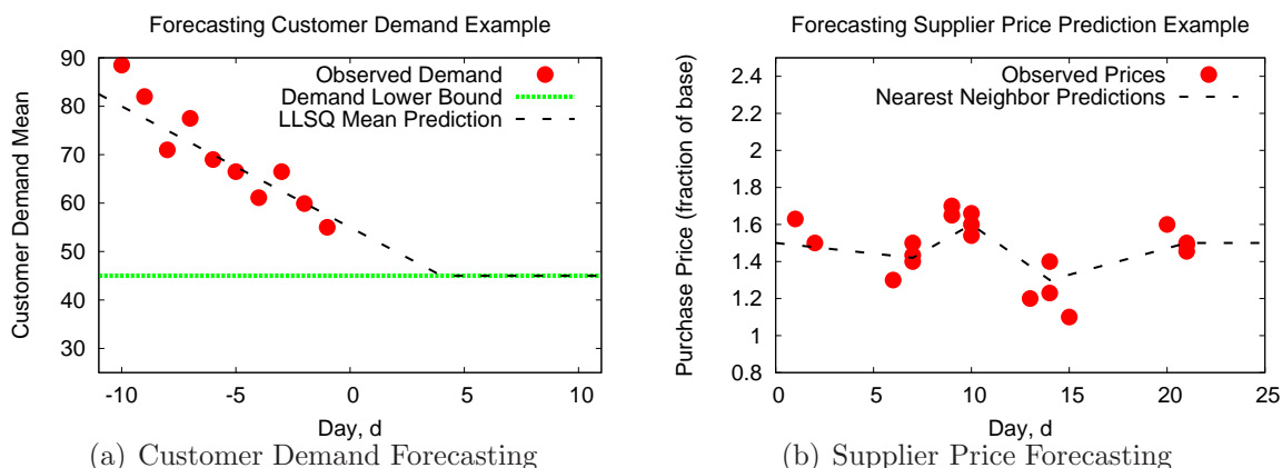
Figure 5: Examples of the techniques used by the forecast module to predict prices.
