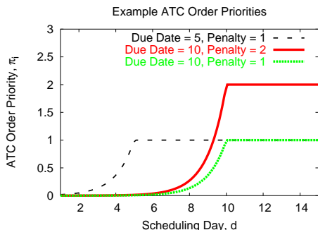
Figure 10: Example of ATC priorities for different orders on different scheduling days ( \alpha = 1 ). Notice that ATC prioritizes by penalty once an order’s due date is reached, and by slack for orders with the same penalty.
