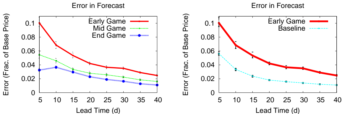
(a) Error in component price forecast as a function of lead time in different game segments. (b) Error of early segment component price prediction with baseline that used unlimited probes.
