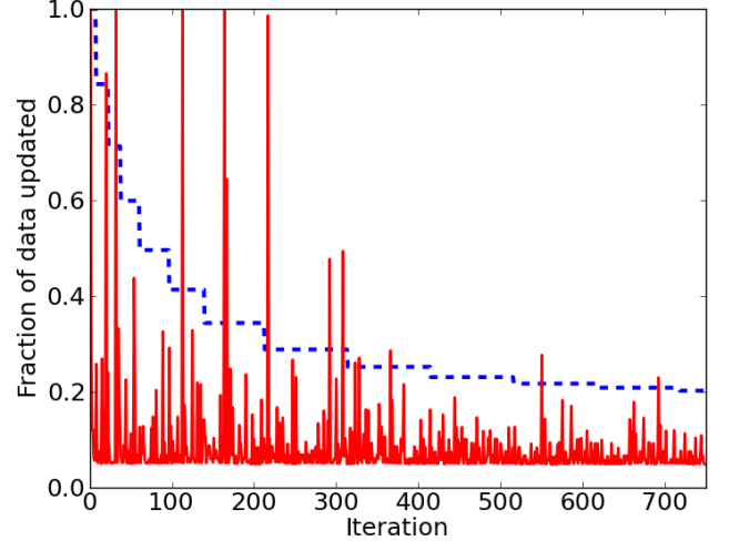
Figure 3: Fraction of data updated by each iteration for the cascade (dashed blue line) and anytime predictor (solid red line).
