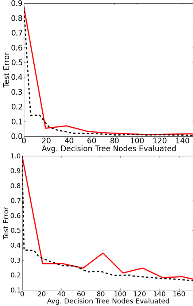
Figure 1: Test set error as a function of prediction time for the UCI ‘pendigits’ (top) and ‘covertypes’ (bottom) dataset. The algorithms shown are SPEEDBOOST.MP (black dashed line), and AdaBoost.MM [7] (red solid line).
