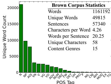
Figure 1: Brown Corpus statistics and count of unique words ( Unique Word Count ) for top 21 Parts-of-Speech tags ( POS Tag ) in the Brown Corpus. N, NP, ADJ, ... correspond to Noun, Noun Proper, Adjective, ... The uneven distribution of word counts among POS tags has important implications on password search space and guessing effort.
