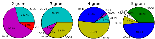
Figure 4: Tag-rules of length 2 to 5 grouped by the size of their search space (in bits or \log_2 ). Numbers outside indicate the range of bits, and numbers inside indicate the percentage of tag-rules with those many bits. Tag-rules divide the password search space unevenly, and many tag-rules have low strength. For example, 8.9% of 3-gram tag-rules have 10-19 bits of strength.
