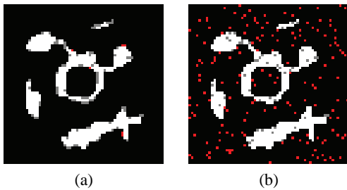
Fig. 1. Comparison of level set estimation and thresholding for a simulated phantom study. (a) Level set estimate for \gamma = 0.70 ; \text{vol}(\Delta(S_\gamma, \hat{S})) = 0.023 . (b) Voxel-wise threshold estimate for \gamma = 0.70 ; \text{vol}(\Delta(S_\gamma, \hat{S})) = 0.051 .
