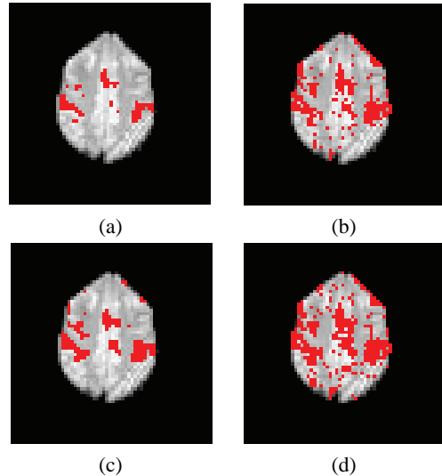
Fig. 2. Estimates of neural activation regions. (a) Level set estimate for \gamma = 0.95 . (b) Voxel-wise threshold estimate for \gamma = 0.95 . (c) Level set estimate for \gamma = 0.90 . (d) Voxel-wise threshold estimate for \gamma = 0.90 . The red regions overlaid onto the anatomic grayscale image represent the declared activity.
