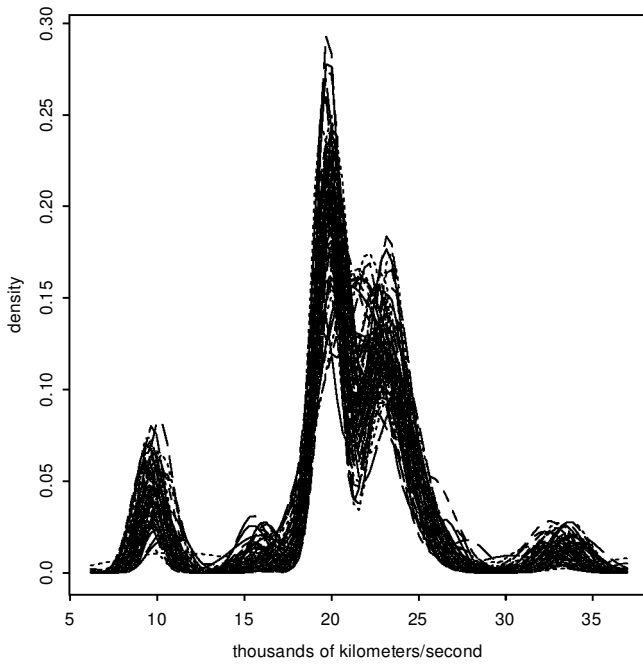
Figure 7. Seventy-five predictive densities (3.2) for the galaxy data selected randomly over 3,500 iterations.
