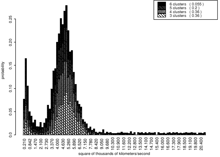
Figure 10. Averaged mixing distribution for the variance distribution based on a uniform prior for \tau_k .
