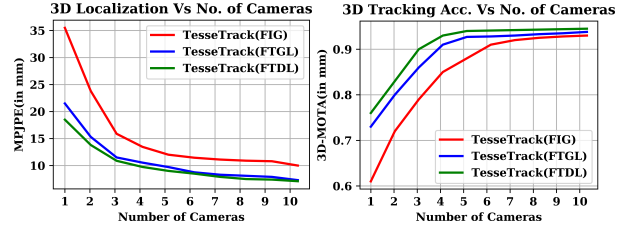
Figure 4: Impact of number of cameras on body joint localization error (MPJPE) (left) and pose tracking accuracy (3D MOTA) (right). TesseTrack (FTDL) shows the greatest advantage with lower number of cameras.
