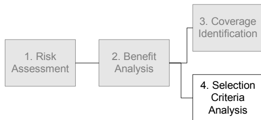
Figure 1 SAEM Steps
