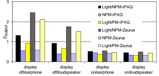
Fig. 3. Ratio of system energy consumptions for text output over speech output under different scenarios
