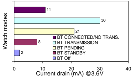
Fig. 8. Power consumption for the watch in different modes
