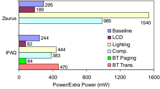
Fig. 1. Baseline power and extra hardware power consumption
