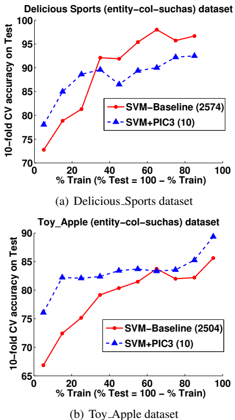
Figure 4: SSL Task : Comparison of SVM+PIC3 vs. SVM-Baseline
