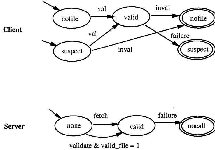
Figure 5: State Transition Graphs for AFS-2
