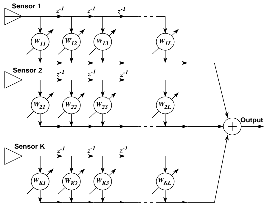
Figure 2-2: Traditional Adaptive Array.
