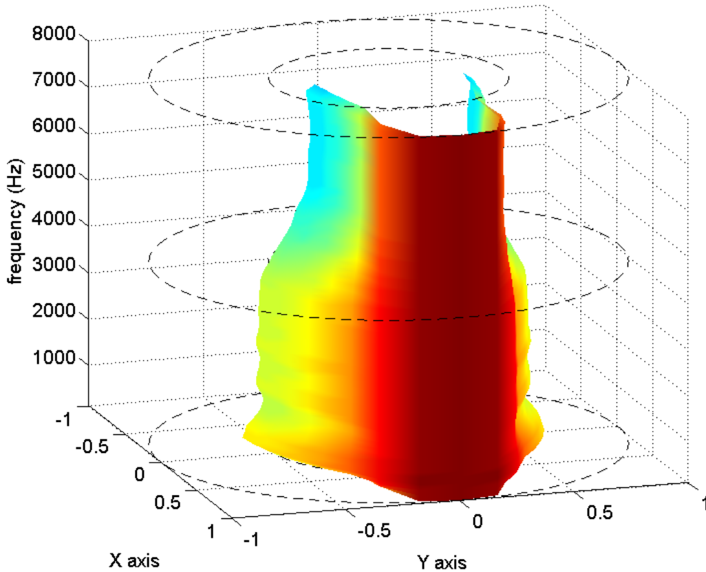
Figure 3.15: Mask presence pattern for two-microphone array with an interfering pink noise signal, d = 4 cm, \phi_T = 20^\circ , SIR = 0 dB (angle in the X-Y plane corresponds to interferer azimuth)
