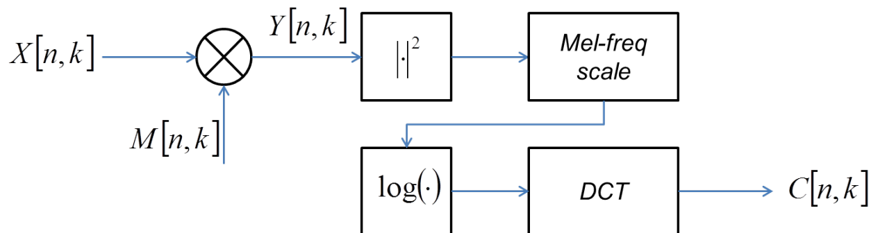
Figure 4.3: Direct MFCC-style feature extraction from the masked signal
