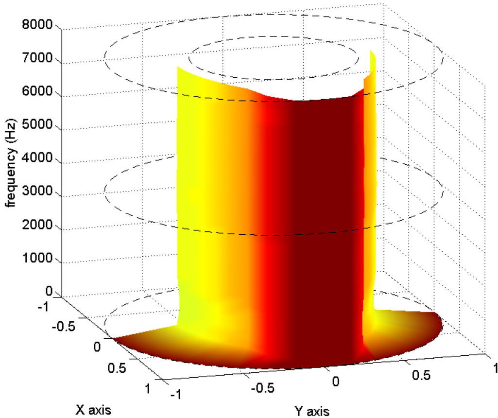
Figure 3.4: Mask presence pattern for two-microphone array, d = 4 cm, \phi_T = 20^\circ , SIR = 10 dB (angle in the X-Y plane corresponds to interferer azimuth)
