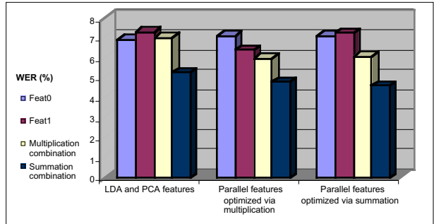
Figure 1: Word error rates (WER) for the DARPA RM corpus obtained using LDA features, PCA features, and optimized features that are derived from them, both individually and in combination. Results are clustered into three blocks according to how the features are generated. Results within each block differ according to whether features are used in isolation or in either additive or multiplicative combination.
