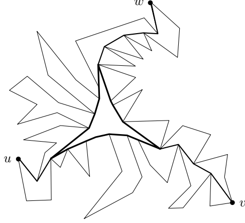
FIGURE 27. A geodesic triangle.
