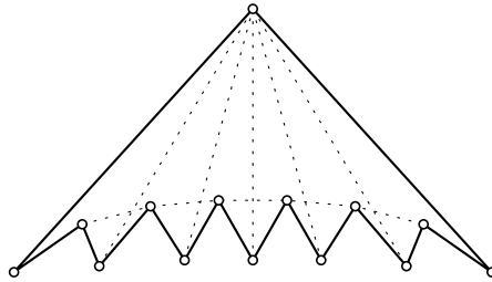
FIGURE 10. A pseudo- k -gon with 2^{k-3} pseudo-triangulations.
