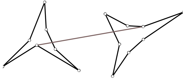
FIGURE 31. Two pseudo-triangles and their unique common tangent.
