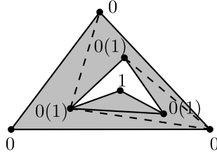
FIGURE 17. In a region R (shaded) that is not simply connected, the folding edges of the highest locally convex function may not create a pseudo-triangulation. The numbers indicate the heights z_i in the lower locally convex hull. The numbers in parentheses indicate the given heights h_i , whenever they are different from the final heights z_i . There is a face at z = 0 which is not a pseudo-triangle. (It is not even a simple polygon.) Perturbing the heights or the vertices will not change this situation.
