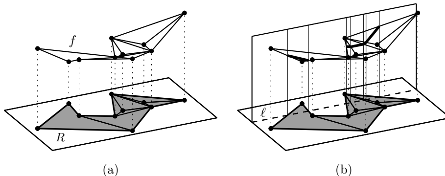
FIGURE 11. (a) A 3D lifting f of a geometric graph (in this case, a pseudo-triangulation) over a plane region R . (b) This lifting is locally convex. Looking at the restriction of f to a line \ell , one sees that f cannot be extended to a convex function over \mathbb{R}^2 .
