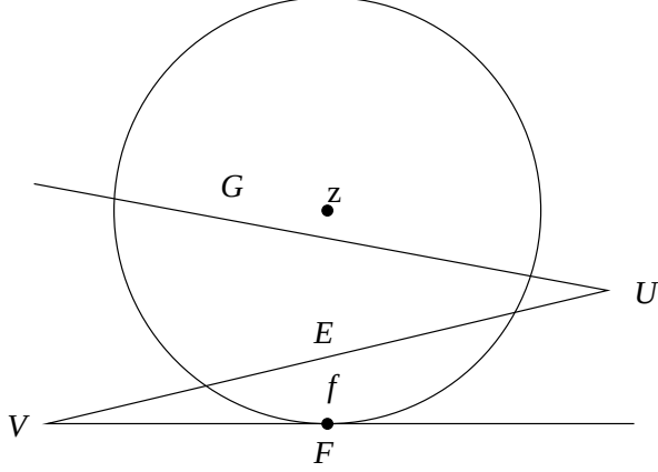
Figure 3: Point z lies in the zone for edge E .
