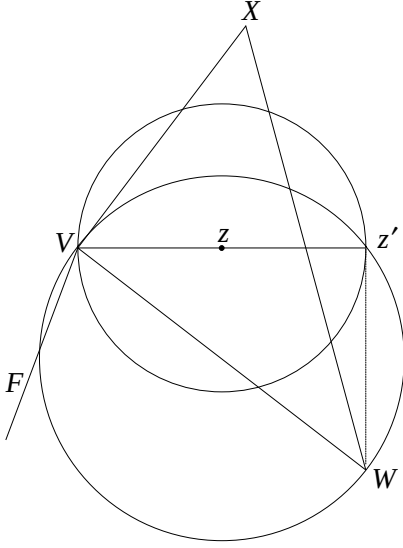
Figure 2: Bounding \text{dist}(z, V) .
