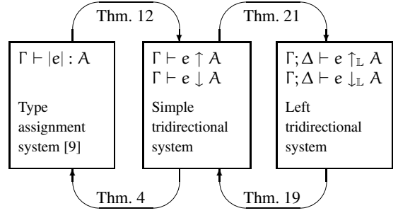
Figure 9: Connections between our type systems
