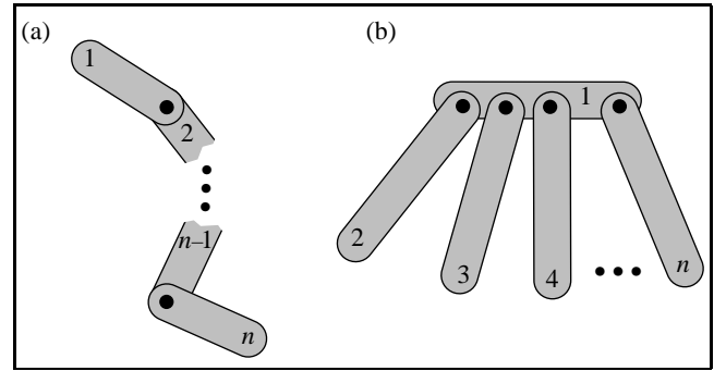
Figure 1: (a) A serial chain. (b) A branched object yielding a completely dense matrix \mathbf{A} = \mathbf{J}\mathbf{M}^{-1}\mathbf{J}^T .
