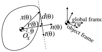
Figure 2: The contact support function (r(\theta), d(\theta))
