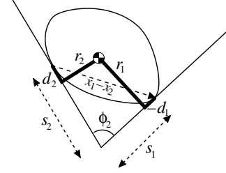
Figure 4: The dependencies between sensor values, the support function and the angle between the palms
