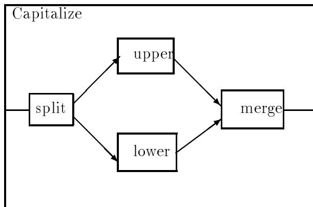
Figure 2: An Architectural Description.
