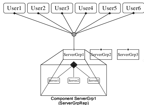
Figure 2. Software Architecture.
