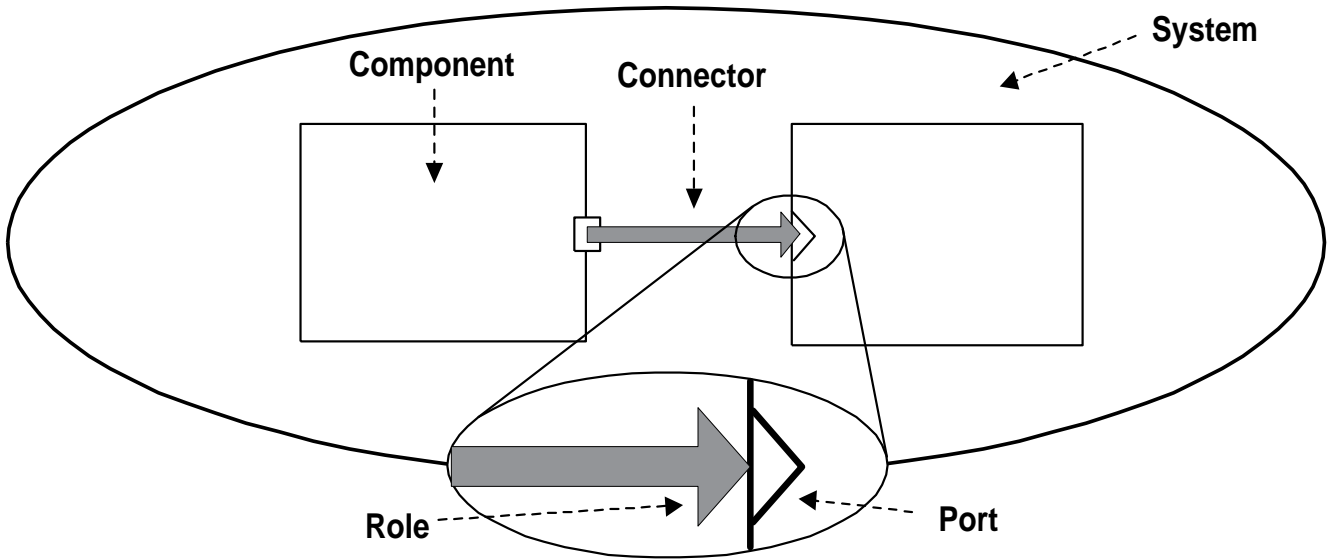
Figure 3: Elements of an ACME Description
