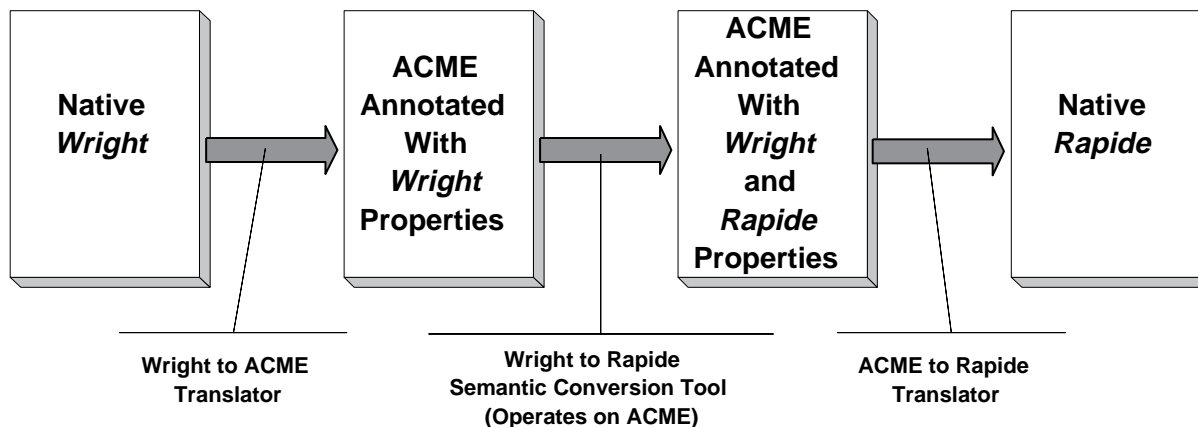
Figure 7: Wright-to-Rapide Translation via ACME
