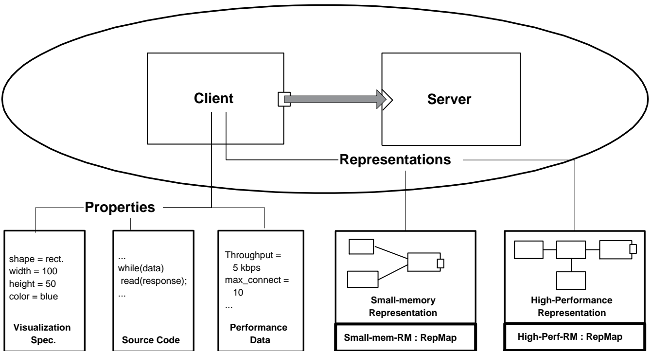
Figure 4: Representations and Properties of a Component
