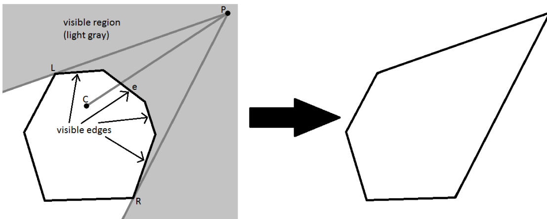
Figure 3: Subroutine BuildTent ( CH, P, e ), with e as the edge intersected by ray CP .
