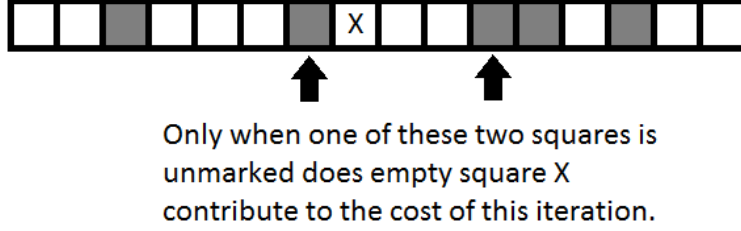
Figure 2: A reversed dart game with 5 darts remaining.
