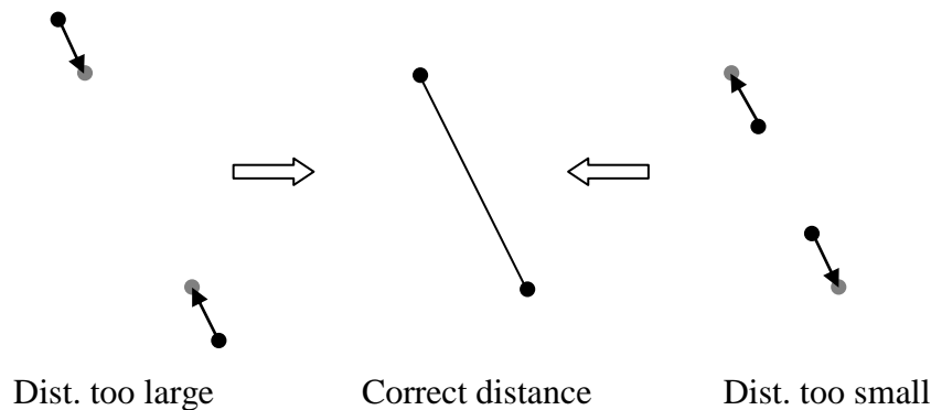
Figure 2. Fixing an invalid distance by moving the particles.
