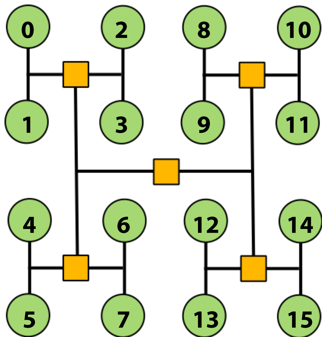
H-Tree
