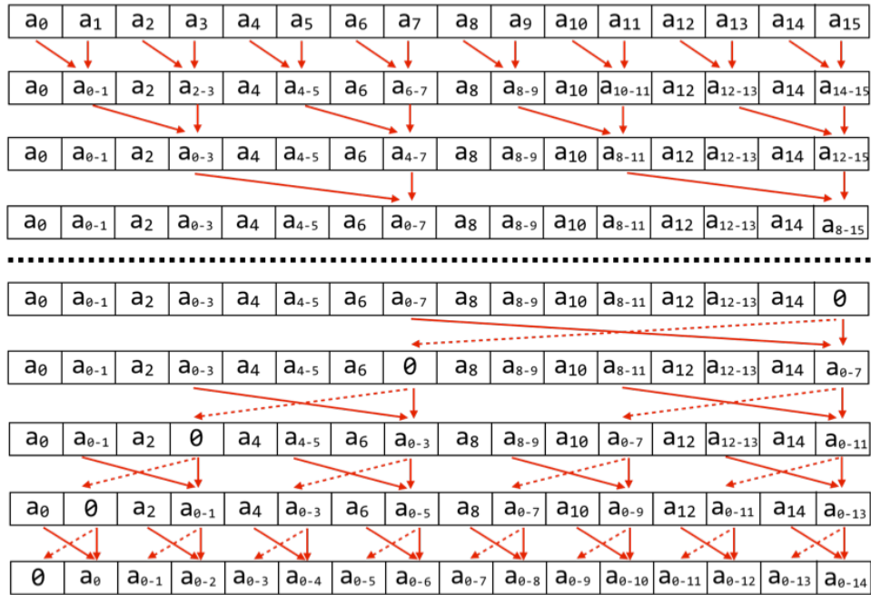
Figure 3: Visualization of exclusive prefix sum for 16 elements
