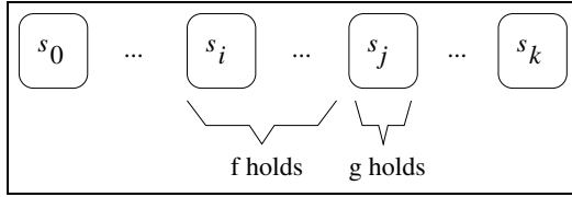
Fig. 13. Translation of \llbracket f \mathbf{U} g \rrbracket_k^i for a loop-free path prefix
