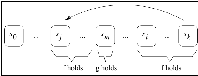
Fig. 16. Translation for a path prefix with a back-loop
