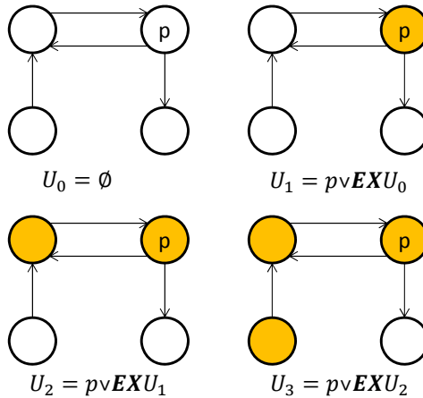
Fig. 7. Example of computing fixed point
