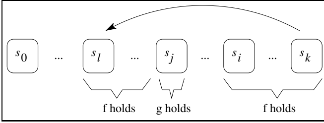
Fig. 14. Translation of \ell[[f \text{ U } g]]_k^i for a path prefix with a back-loop
