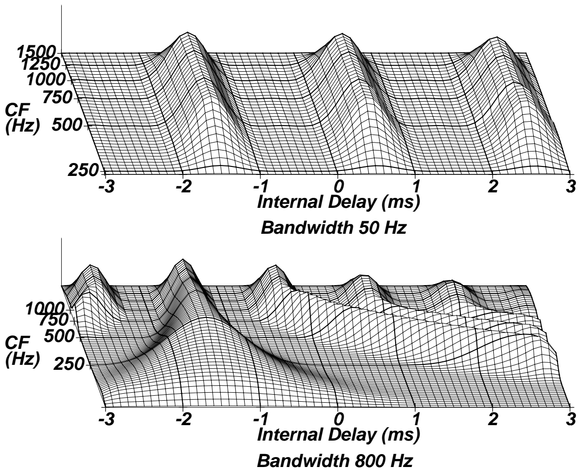
Figure 7. The response of an ensemble of coincidence-counting units to low-frequency band-pass noise with a center frequency of 500 Hz and an ITD of -1.5 ms. Upper panel: response to bandpass noise with a bandwidth of 50 Hz. Lower panel: response to bandpass noise with a bandwidth of 800 Hz.
