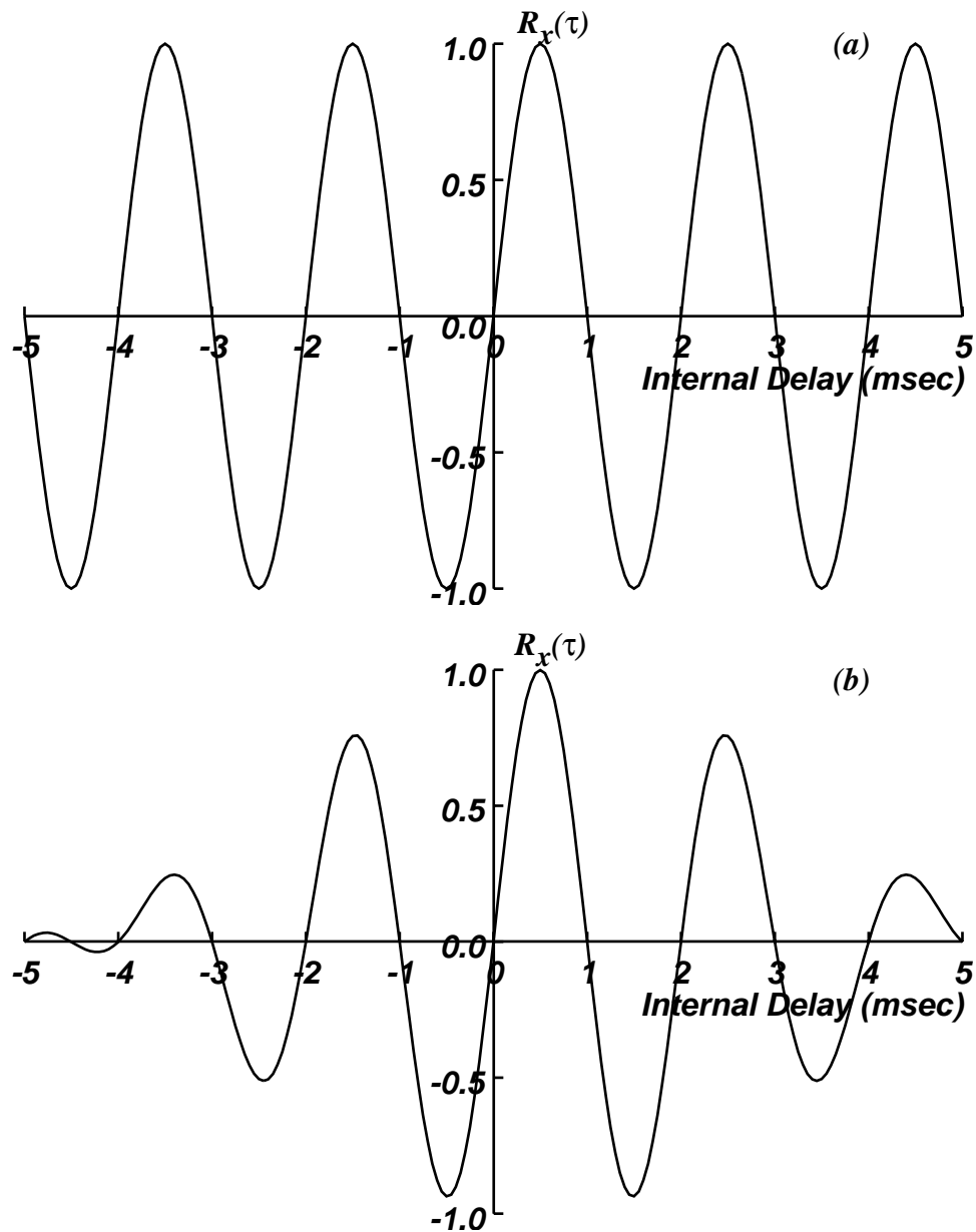
Figure 3. Examples of cross-correlation functions for (a) a 500-Hz pure tone, and (b) band-pass noise with a center frequency of 500 Hz and bandwidth of 200 Hz. In each case the signals are presented with an ITD of 0.5 ms.
