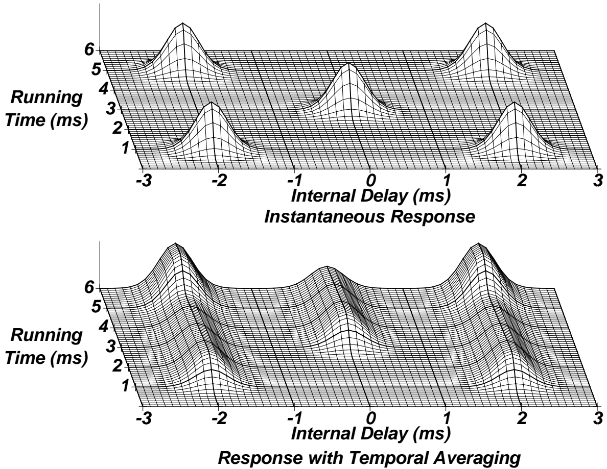
Figure 4. The expected value of the instantaneous number of coincidences, E[L(t, \tau, f)] , as a simultaneous function of running time t and internal delay \tau , to a 500-Hz tone with zero ITD. The response is shown using no temporal integration (upper panel) and using temporal integration by an exponentially-shaped temporal weighting function with an effective cutoff frequency of 5 Hz in the frequency domain.
