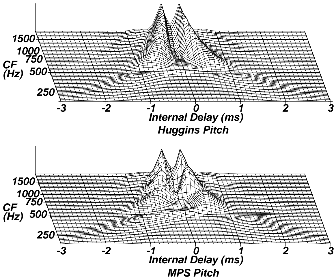
Figure 12. Upper panel: response of an ensemble of coincidence-counting units to a “Huggins-pitch” stimulus with an interaural phase transition from -\pi to \pi radians occurring in a narrow range of frequencies about 500 Hz. Lower panel: response of an ensemble of coincidence-counting units to a multiple-phase-shift (MPS) stimulus producing dichotic pitch perceptions at 500 Hz. These plots include the effects of the relative number of fiber pairs, as specified by the function p(\tau, f) .
