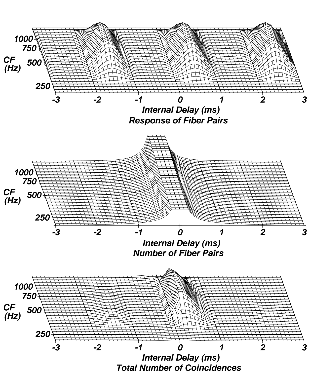
Figure 5. Cross-correlation patterns showing the response of an ensemble of binaural fiber pairs to a 500-Hz pure tone with a 0.5-ms ITD. Upper panel: the relative number of coincidences per fiber pair as a function of internal delay \tau (in ms) and CF of the auditory-nerve fibers (in Hz). Central panel: the function p(\tau, f) , which describes the assumed distribution of internal delays as a function of CF. Lower panel: E[L_T(\tau, f)] the expected total number of coincidences as a function of internal delay and CF, which is the product of the upper and central panel.
