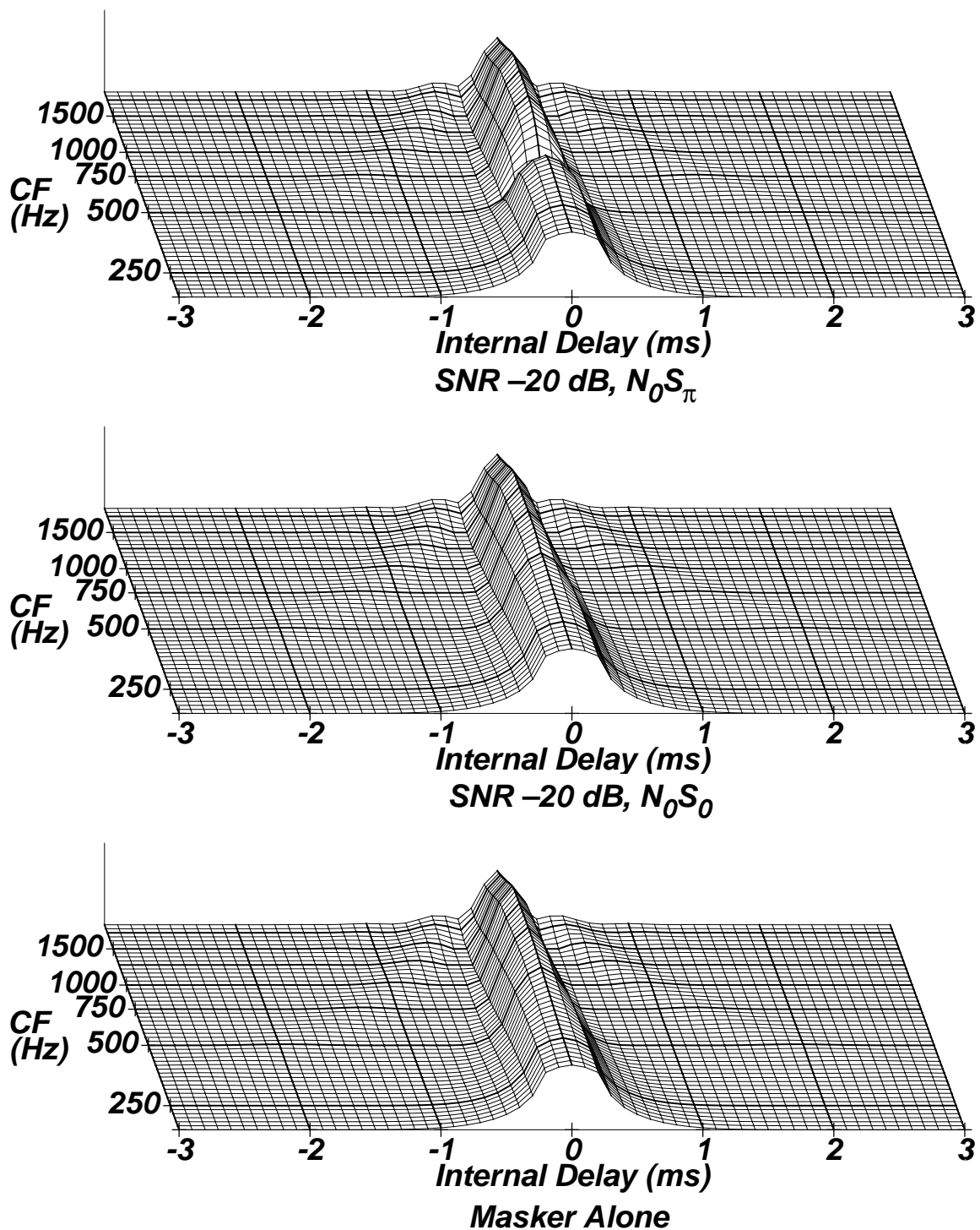
Figure 11. Patterns of coincidence-counting activity showing the response to stimuli used in N_0 S_\pi and N_0 S_0 binaural masking-level difference experiments. The target is presented at 500 Hz, either interaurally in phase or out of phase, as indicated, and the masker is broadband diotic noise. These plots include the effects of the relative number of fiber pairs, as specified by the function p(\tau, f) .
