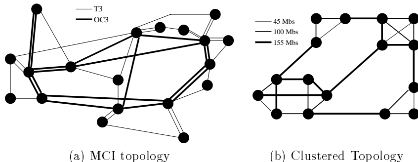
Figure 1 Topologies
