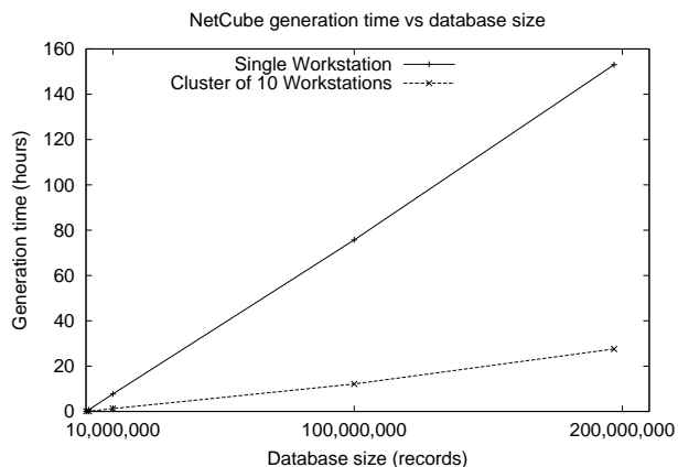
Figure 7: Build time for the set of multiple BNs increases linearly with the number of records in the database. Moreover, parallelization over a number of workstation scales the build time down linearly. Each partition of the database contains 100,000 records and can be processed independently of others.
