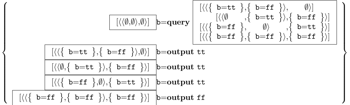
Figure 9: The algorithm \mathbf{gf} for gf
