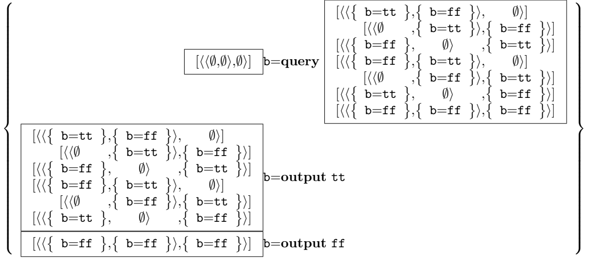
Figure 10: The algorithm gf' for gf'
