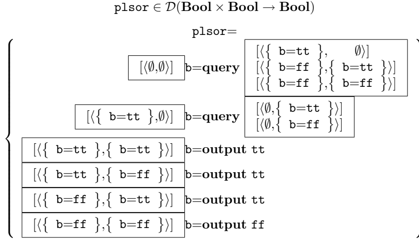
Figure 7: The algorithm \text{plsor} for \text{sor}
