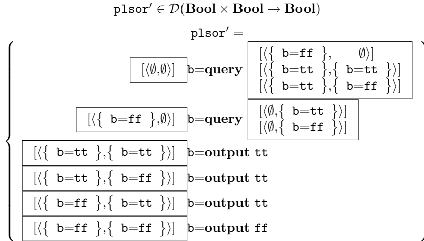
Figure 8: The algorithm \text{plsor}' for \text{sor}
