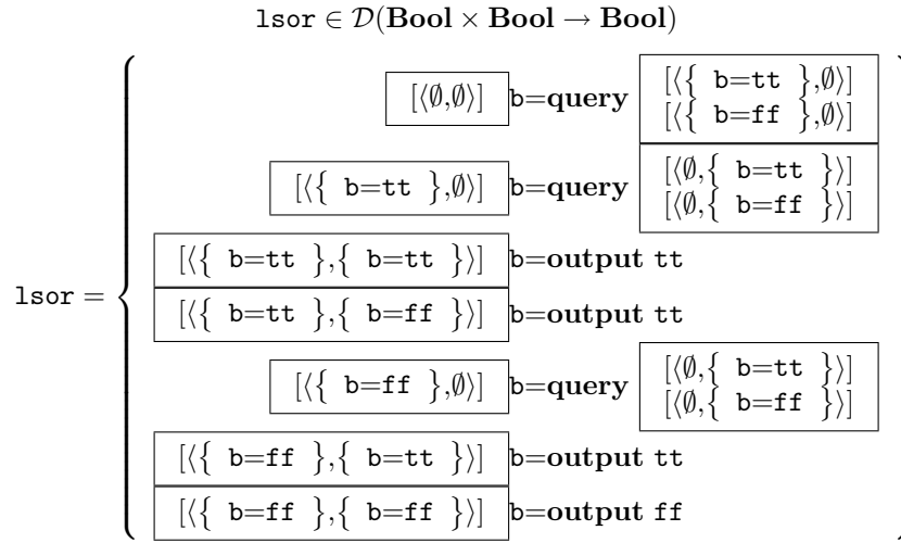
Figure 5: The algorithm lsor for sor
