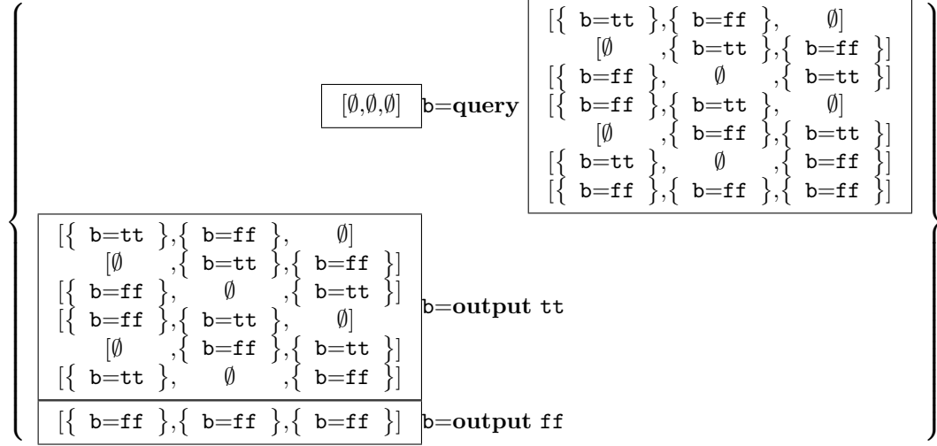
Figure 14: The curried algorithm for gf' , \text{cgf}' = \text{curry}(\text{curry}(gf'))
