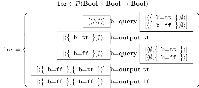
Figure 3: The algorithm lor for lor
