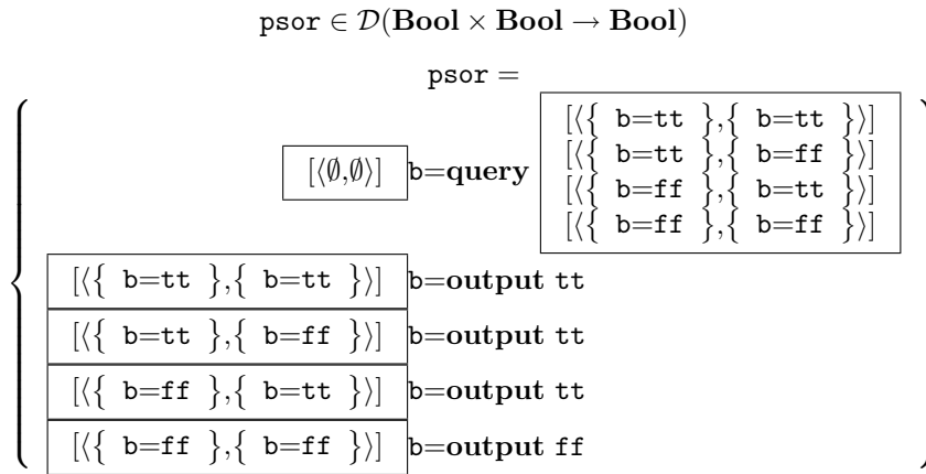
Figure 6: The algorithm psor for sor
