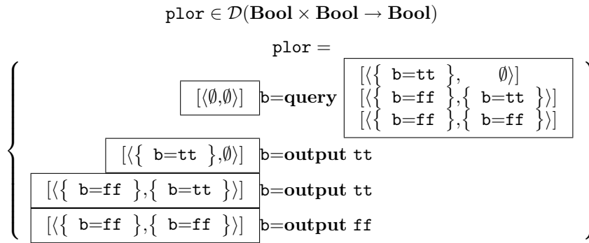
Figure 4: The algorithm plor for lor
