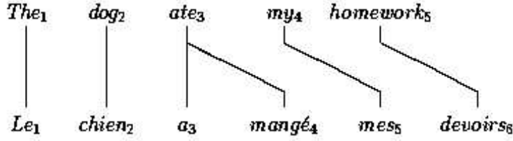
Figure 3: drawLines representation
