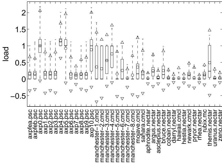
Figure 4: Statistical summary of load traces.
