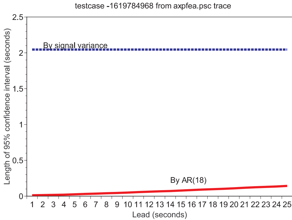
Figure 2: Benefits of prediction: interactive cluster machine with long term load average of 0.17.
