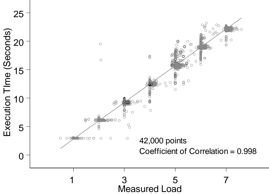
Figure 3: Relationship between average load during execution and execution time
