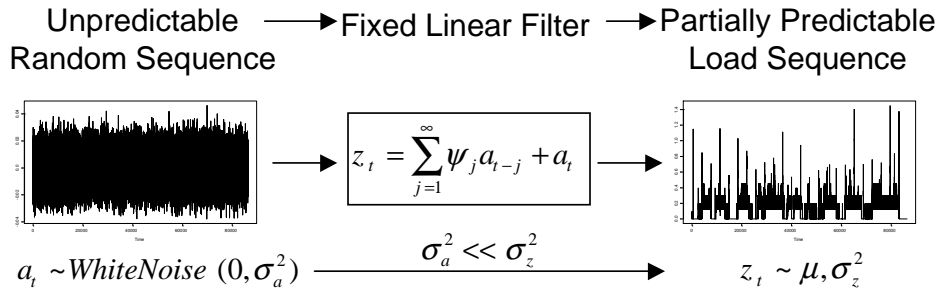
Figure 6: Linear time series models for load prediction.
