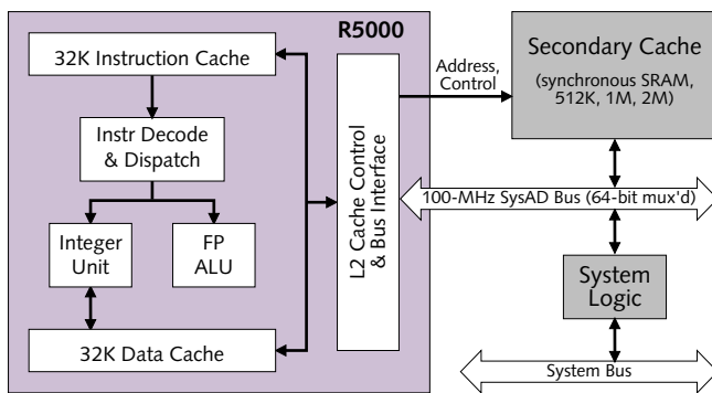
Figure 1. The R5000 contains a simple superscalar core and large on-chip caches. It also directly controls an external cache.
