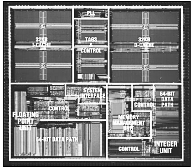
Figure 2. IDT's version of the R5000 contains 3.6 million transistors and is built in a 0.35-micron CMOS process with three metal layers and two poly layers; it measures 8.7 \times 9.7 mm ( 84 \text{ mm}^2 ). Other vendors' versions vary slightly in size and transistor count.
