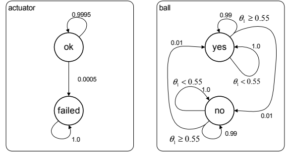
Figure 2: Discrete transition model for an acrobatic robot. If the actuator has failed, it exerts no torque. When the robot catches the ball, \text{ball}=\text{yes} , and the mass of the lower link increases.
