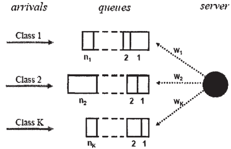
Figure 2: A queue operating under GPS
