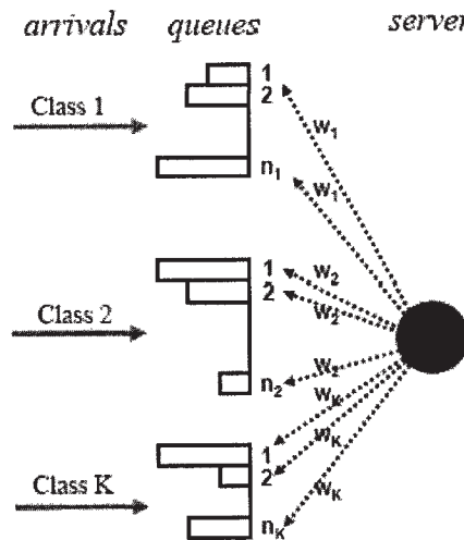
Figure 1: A queue operating under DPS
