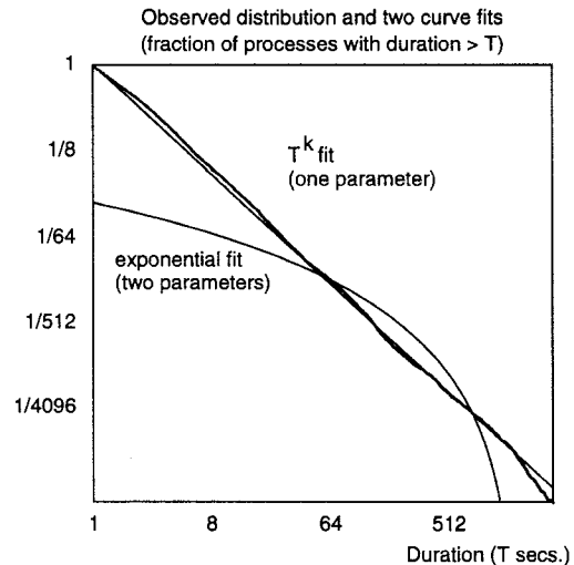
Figure 2: In log-log space, this plot shows the distribution of lifetimes for the \sim 13000 processes with lifetimes > 1 second from our trace-driven simulation (see Section 5), and two attempts to fit a curve to this data. One of the fits is based on the model proposed in this paper, T^k . The other fit is an exponential curve, c \cdot e^{-\lambda T} . Although the exponential curve is given the benefit of an extra free parameter, it fails to model the observed data. The proposed model fits well. Both fits were performed by iteratively-weighted least squares.
