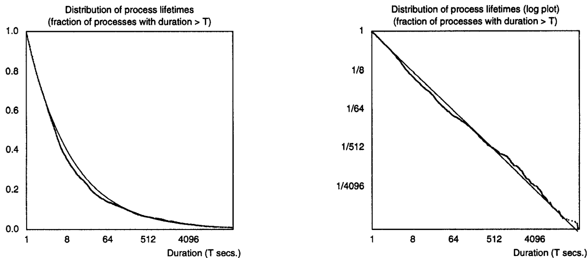
Figure 1: Distribution of process lifetimes for processes with lifetimes greater than 1 second, observed on machine “po” mid-semester. The dotted (thicker) line shows the measured distribution; the solid (thinner) line shows the least squares curve fit. To the right: the same distribution shown on a log-log scale. The straight line in log-log space indicates that the process lifetime distribution can be modeled by T^k , where k is the slope of the line.
