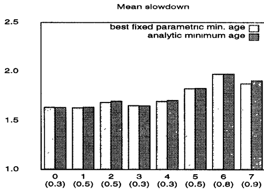
Figure 6: The mean slowdown for eight runs, using the two criteria for minimum migration age. The value of the best fixed parameter \alpha is shown in parentheses for each run.
