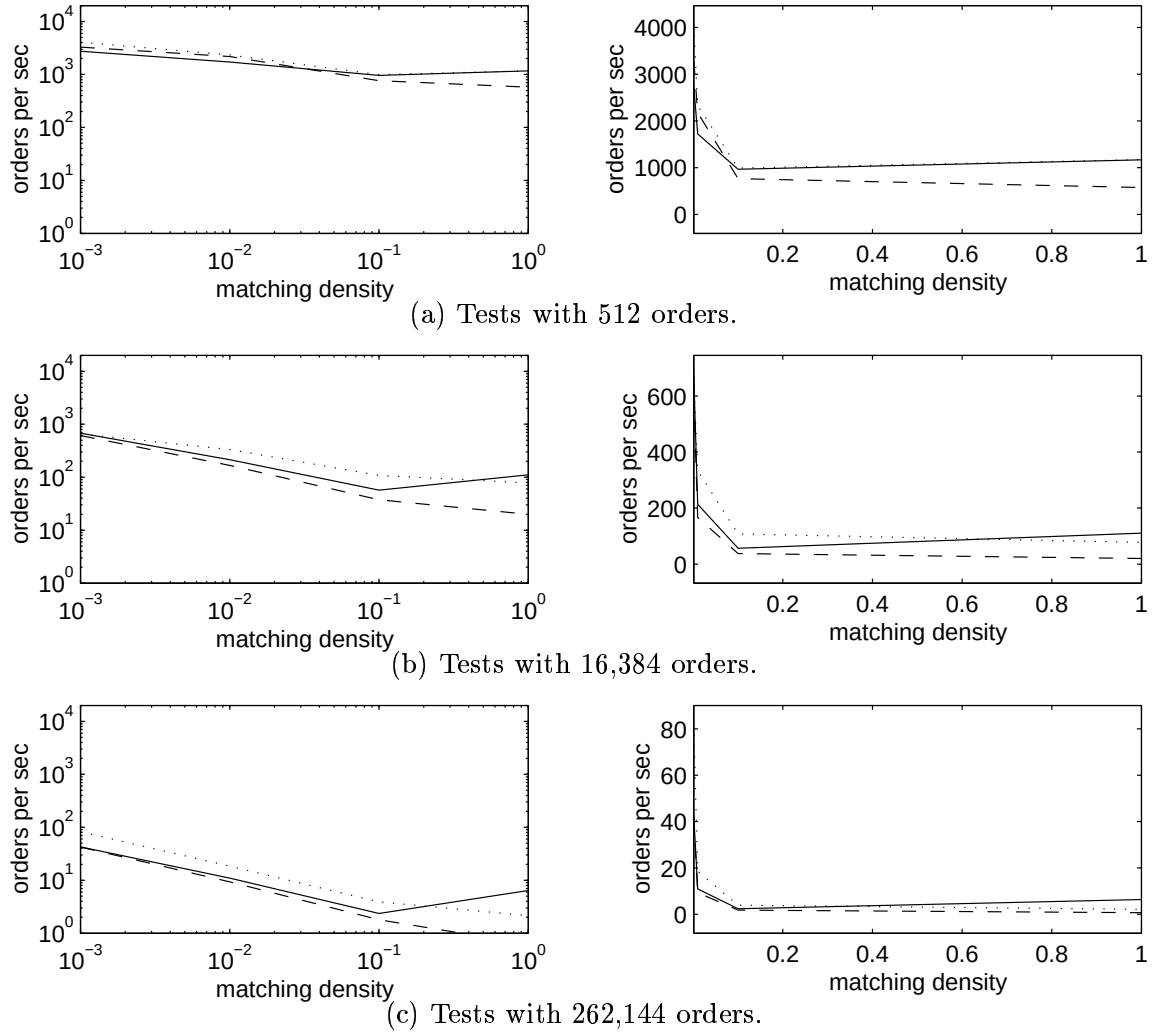
Figure 6.22: Dependency of the throughput on the matching density. The legend is the same as in Figure 6.17.
