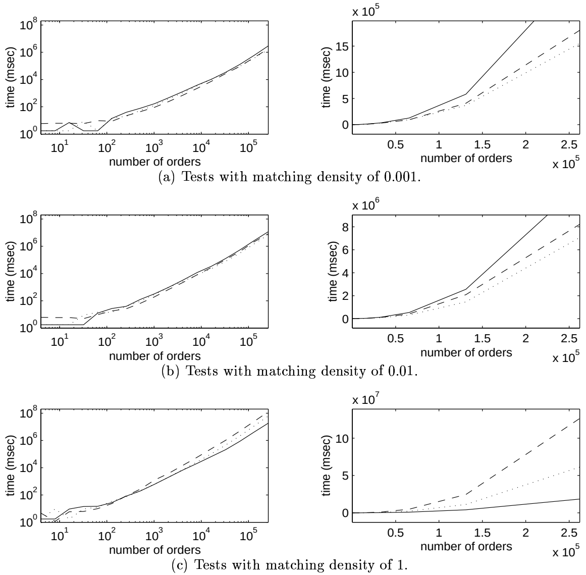
Figure 6.18: Dependency of the response time on the number of orders. The legend is the same as in Figure 6.17.
