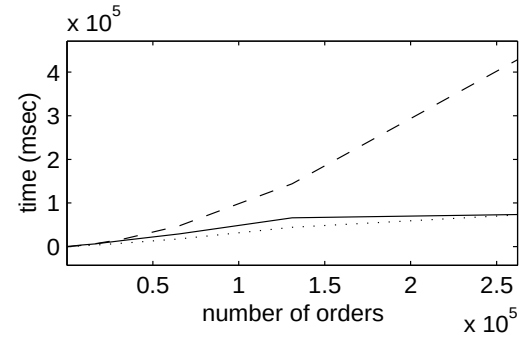
(b) Tests with three attributes, sixteen values per attribute, and matching density of 0.01.
