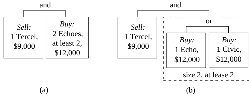
Figure 2.13: Examples of size specifications in conjunctive orders.
