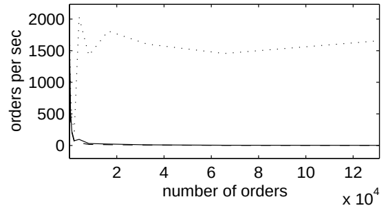
(c) Tests with ten attributes, 1,024 values per attribute, and matching density of 1.
