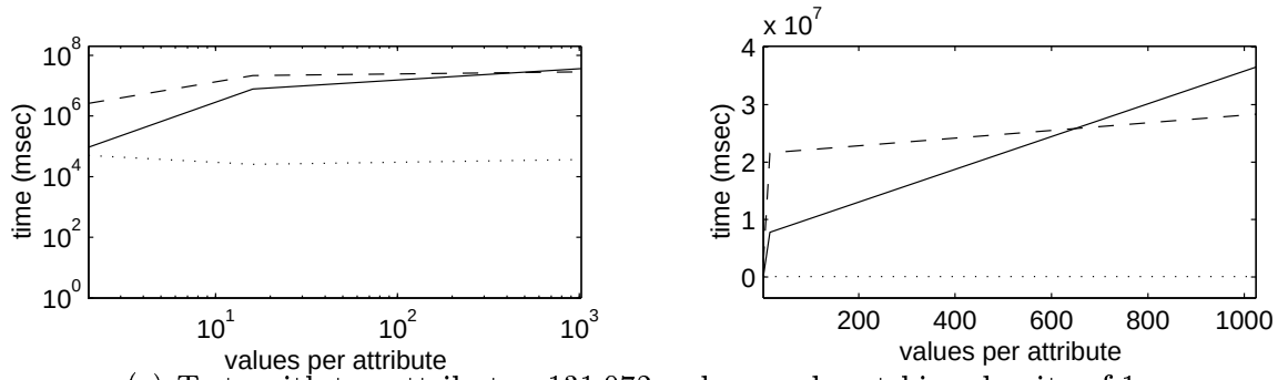
(c) Tests with ten attributes, 131,072 orders, and matching density of 1.
