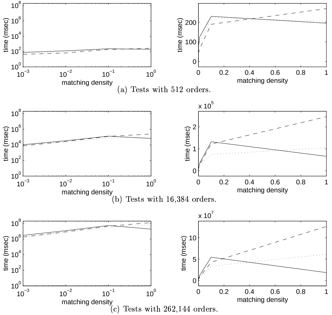
Figure 6.21: Dependency of the response time on the matching density. The legend is the same as in Figure 6.17.
