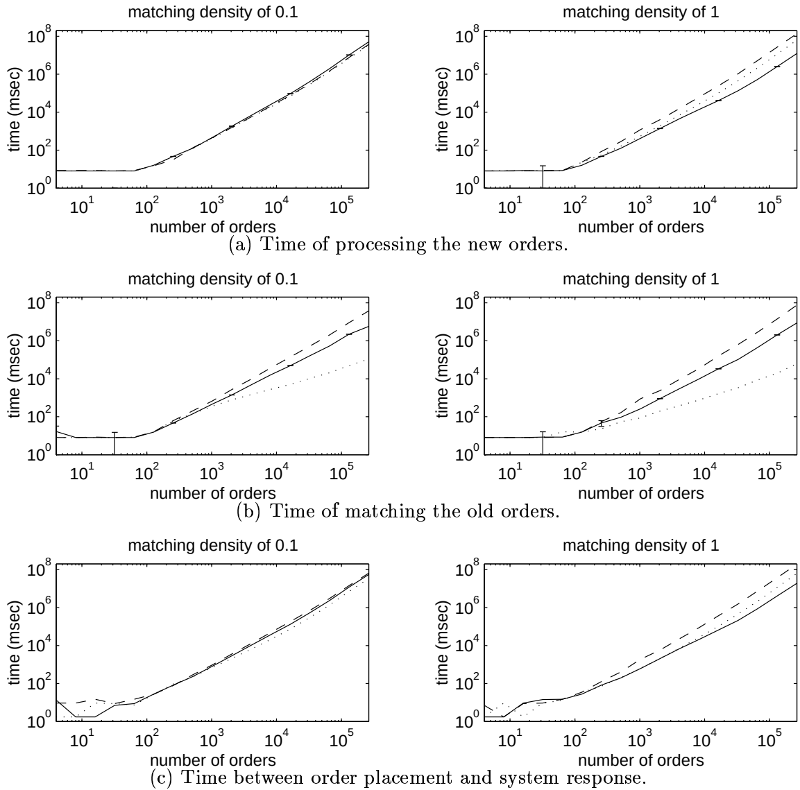
Figure 6.16: Performance in the car market for matching density of 0.1 (left) and 1 (right). The legend is the same as in Figure 6.15.
