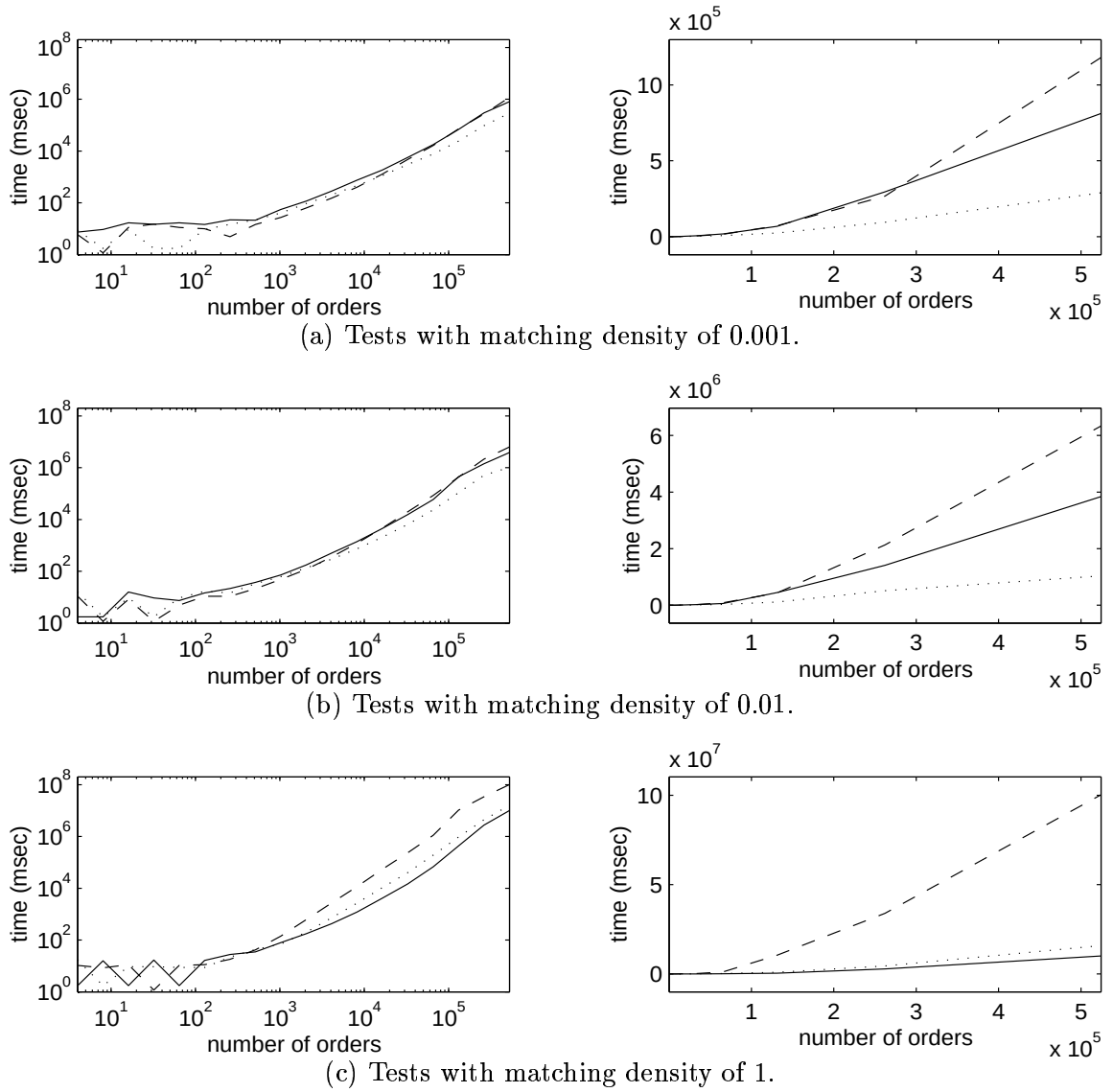
Figure 6.26: Dependency of the response time on the number of orders. The legend is the same as in Figure 6.25.
