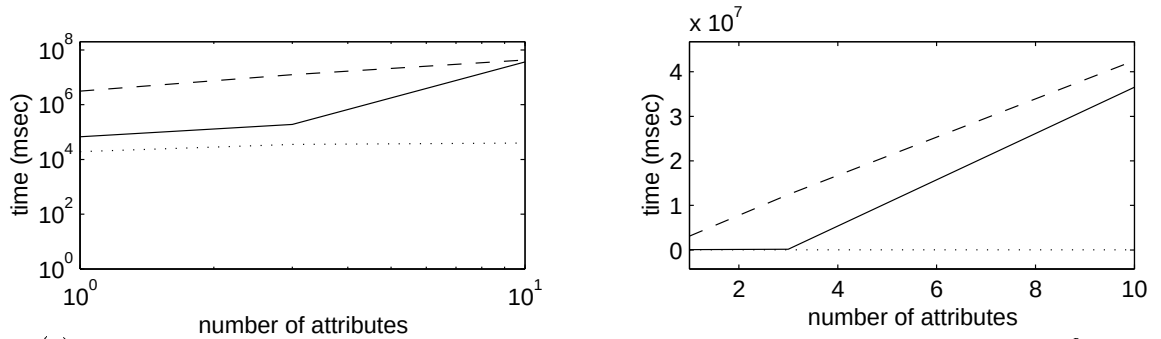
(c) Tests with 1,024 values per attribute, 131,072 orders, and matching density of 1.
