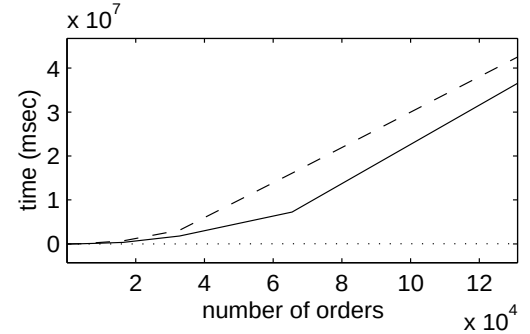
(c) Tests with ten attributes, 1,024 values per attribute, and matching density of 1.
