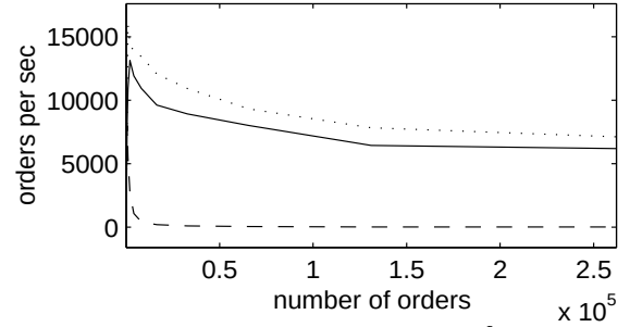
(a) Tests with one attribute, two values per attribute, and matching density of 0.001.
