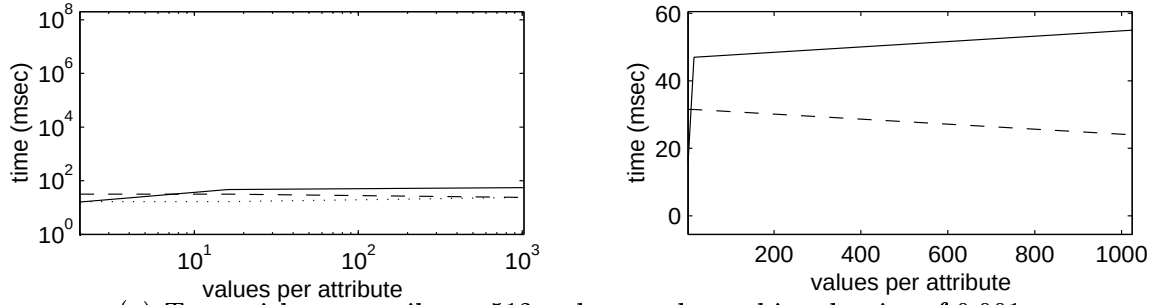
(a) Tests with one attribute, 512 orders, and matching density of 0.001.
