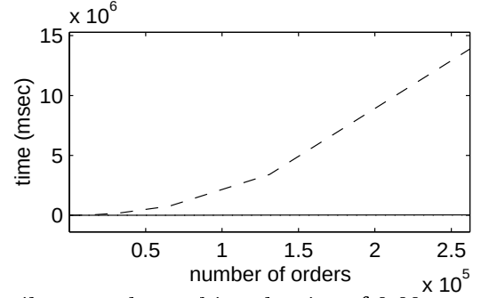
(a) Tests with one attribute, two values per attribute, and matching density of 0.001.
