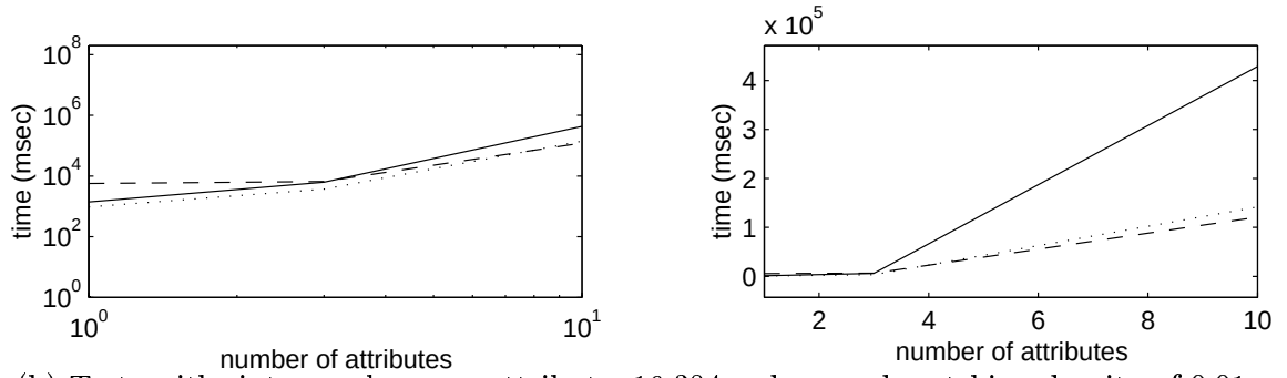
(b) Tests with sixteen values per attribute, 16,384 orders, and matching density of 0.01.
