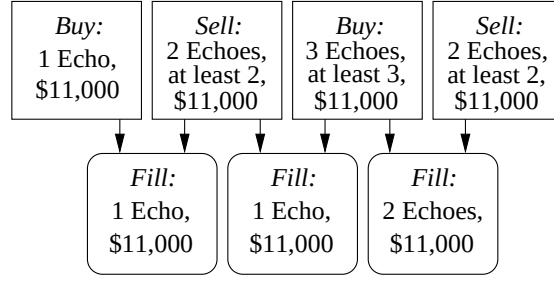
Figure 2.6: Example of a transaction that involves multiple buy and sell orders.
