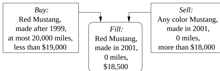
Figure 1.1: Matching orders and the resulting trade. When the system finds a match between two orders, it generates a fill, which is a trade that satisfies both parties.
