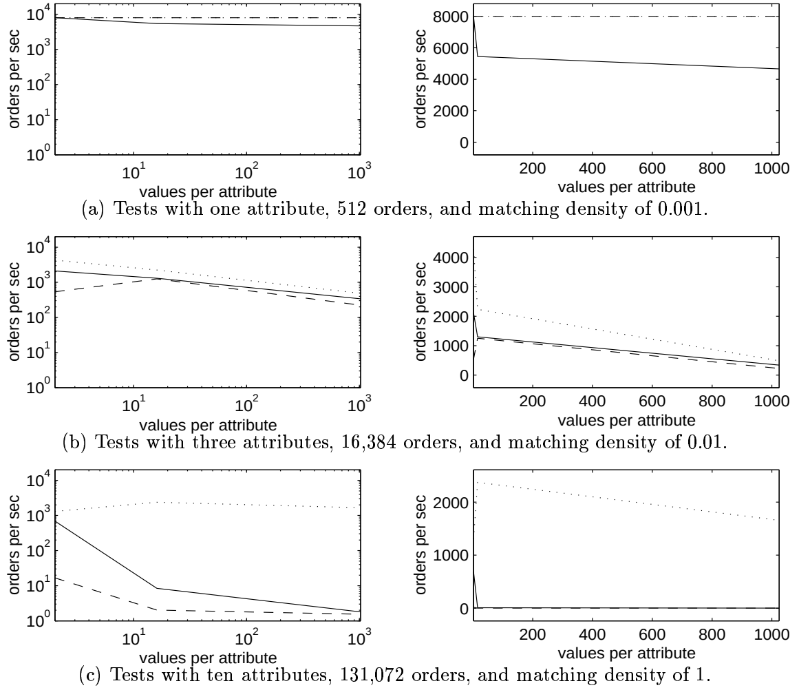
Figure 6.9: Dependency of the throughput on the number of values per attribute. The legend is the same as in Figure 6.1.
