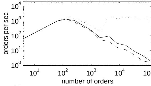
(c) Tests with ten attributes, 1,024 values per attribute, and matching density of 1.
