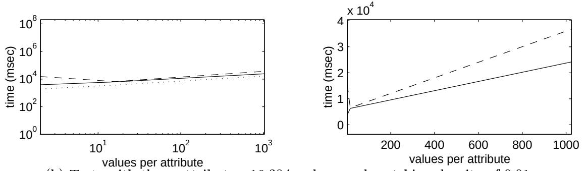
(b) Tests with three attributes, 16,384 orders, and matching density of 0.01.
