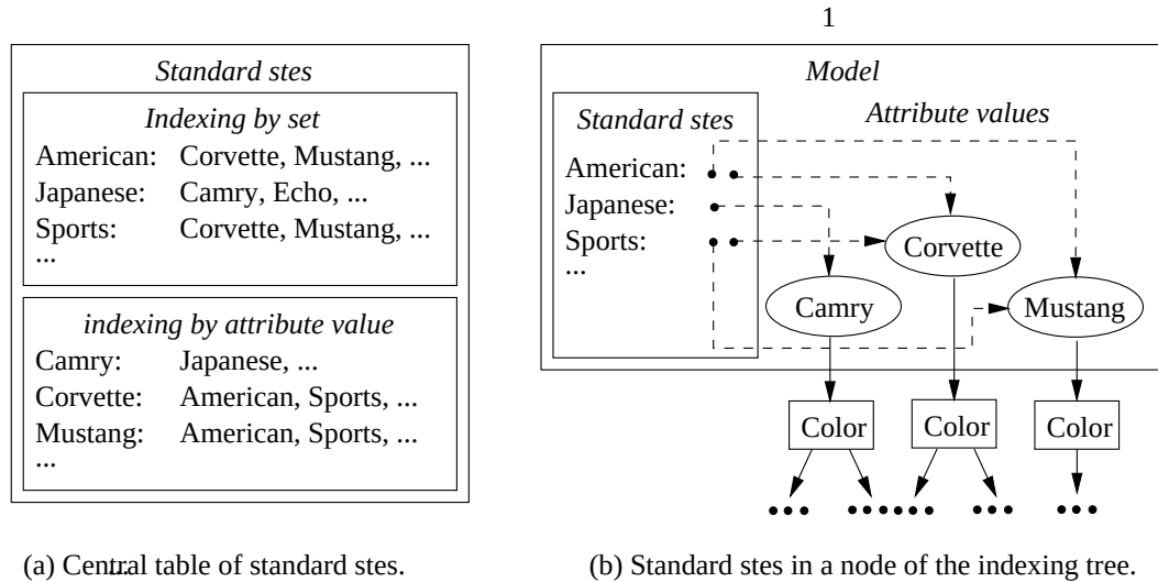
Figure 4.11: Standard sets of values. The market includes a central table of sets (a), and every node in the indexing tree includes a table of sets for the respective attribute (b).
