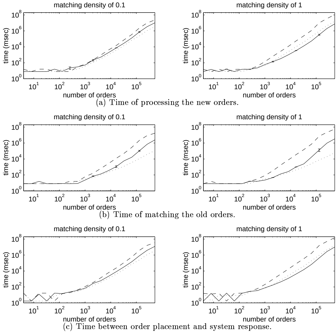
Figure 6.24: Performance in the commercial-paper market for matching density of 0.1 (left) and 1 (right). The legend is the same as in Figure 6.23.
