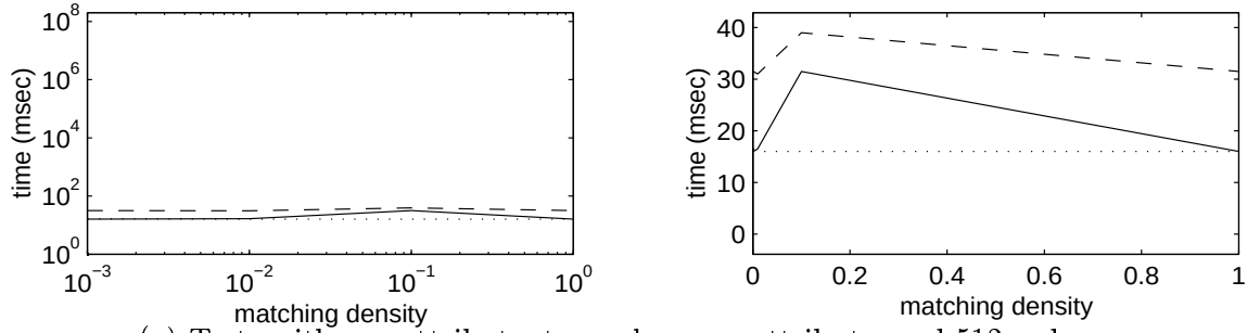
(a) Tests with one attribute, two values per attribute, and 512 orders.
