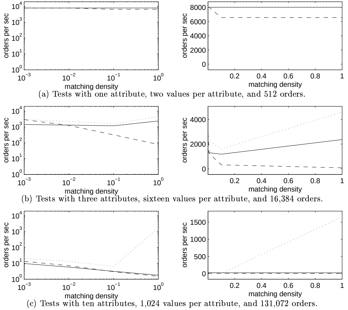
Figure 6.12: Dependency of the throughput on the matching density. The legend is the same as in Figure 6.1.
