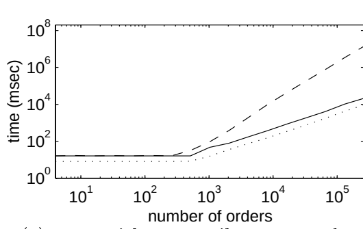
(a) Tests with one attribute, two values per attribute, and matching density of 0.001.
