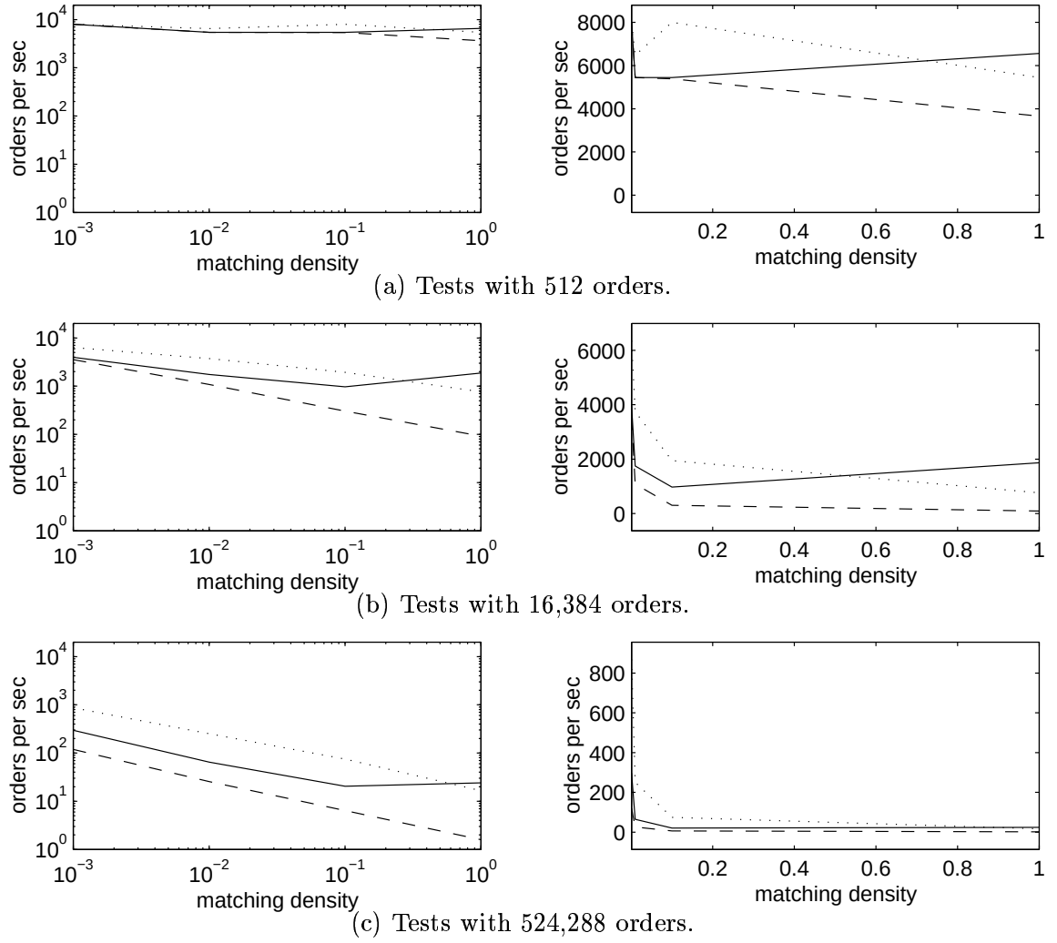
Figure 6.30: Dependency of the throughput on the matching density. The legend is the same as in Figure 6.25.
