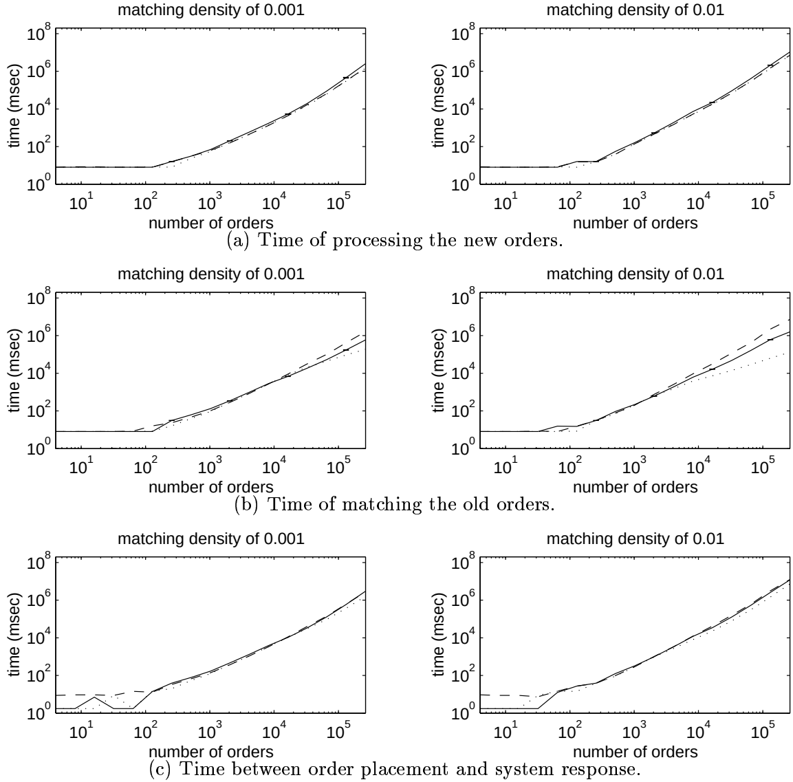
Figure 6.15: Performance in the car market for matching density of 0.001 (left) and 0.01 (right). We show the performance of the best-first search (solid lines), depth-first search that identifies all matches (dashed lines), and depth-first search with a limit on the number of matches (dotted lines).
