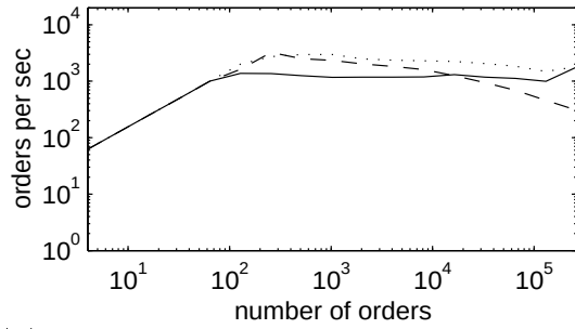
(b) Tests with three attributes, sixteen values per attribute, and matching density of 0.01.
