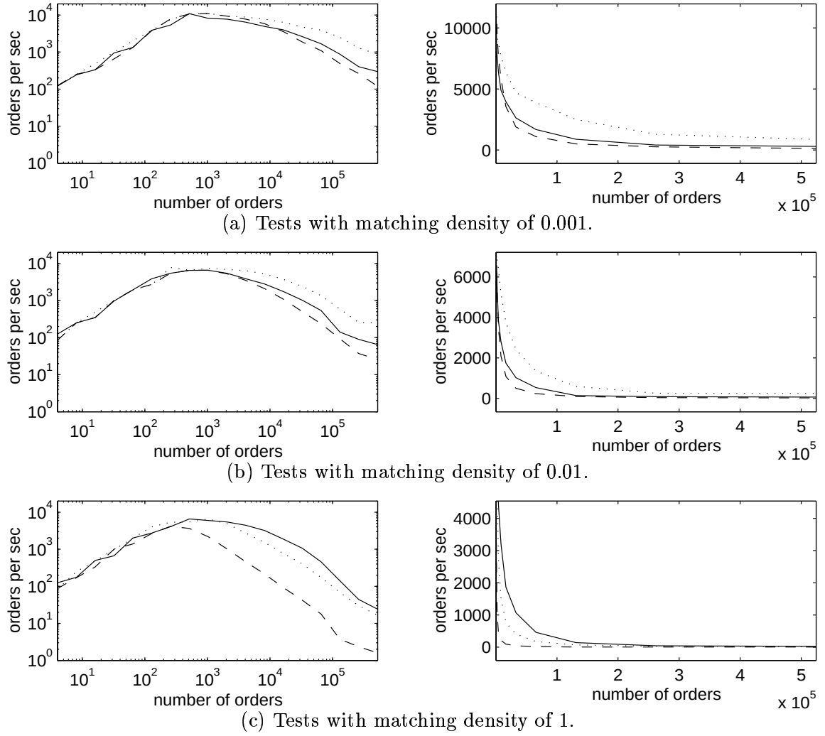
Figure 6.27: Dependency of the throughput on the number of orders. The legend is the same as in Figure 6.25.
