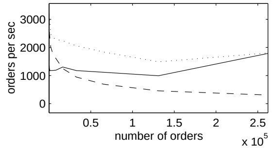
(b) Tests with three attributes, sixteen values per attribute, and matching density of 0.01.
