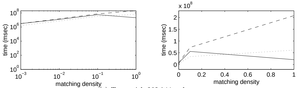
(c) Tests with 262,144 orders.
