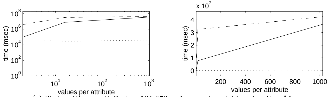
(c) Tests with ten attributes, 131,072 orders, and matching density of 1.
