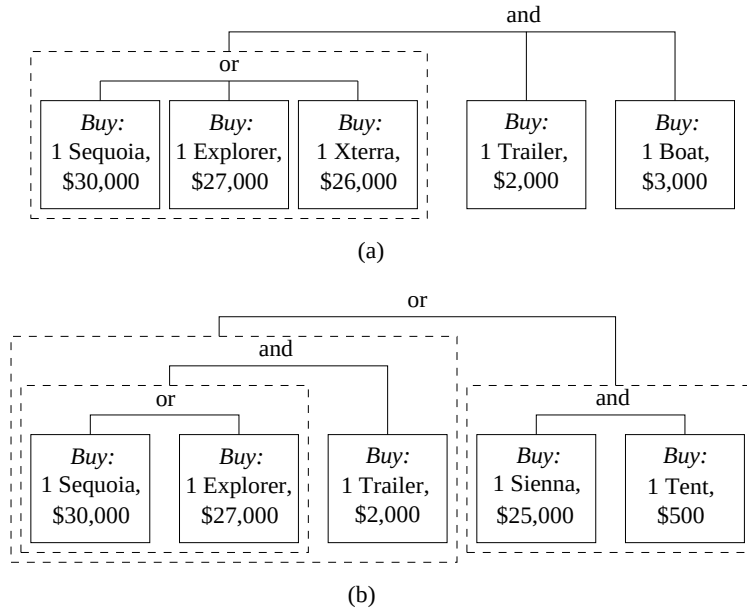
Figure 2.12: Examples of nested disjunctions and conjunctions.
