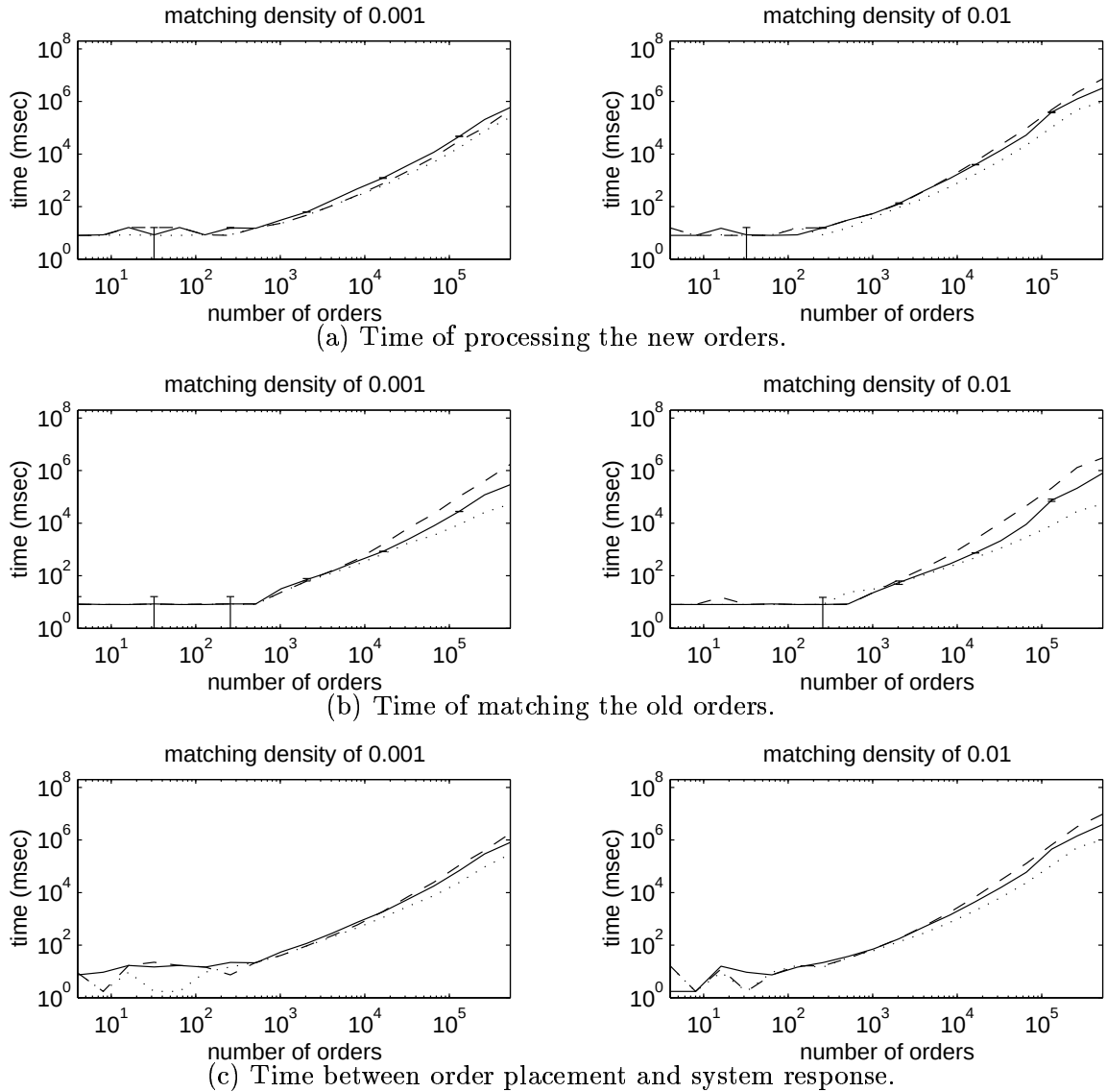
Figure 6.23: Performance in the commercial-paper market for matching density of 0.001 (left) and 0.01 (right). We show the performance of the best-first search (solid lines), depth-first search that identifies all matches (dashed lines), and depth-first search with a limit on the number of matches (dotted lines).
