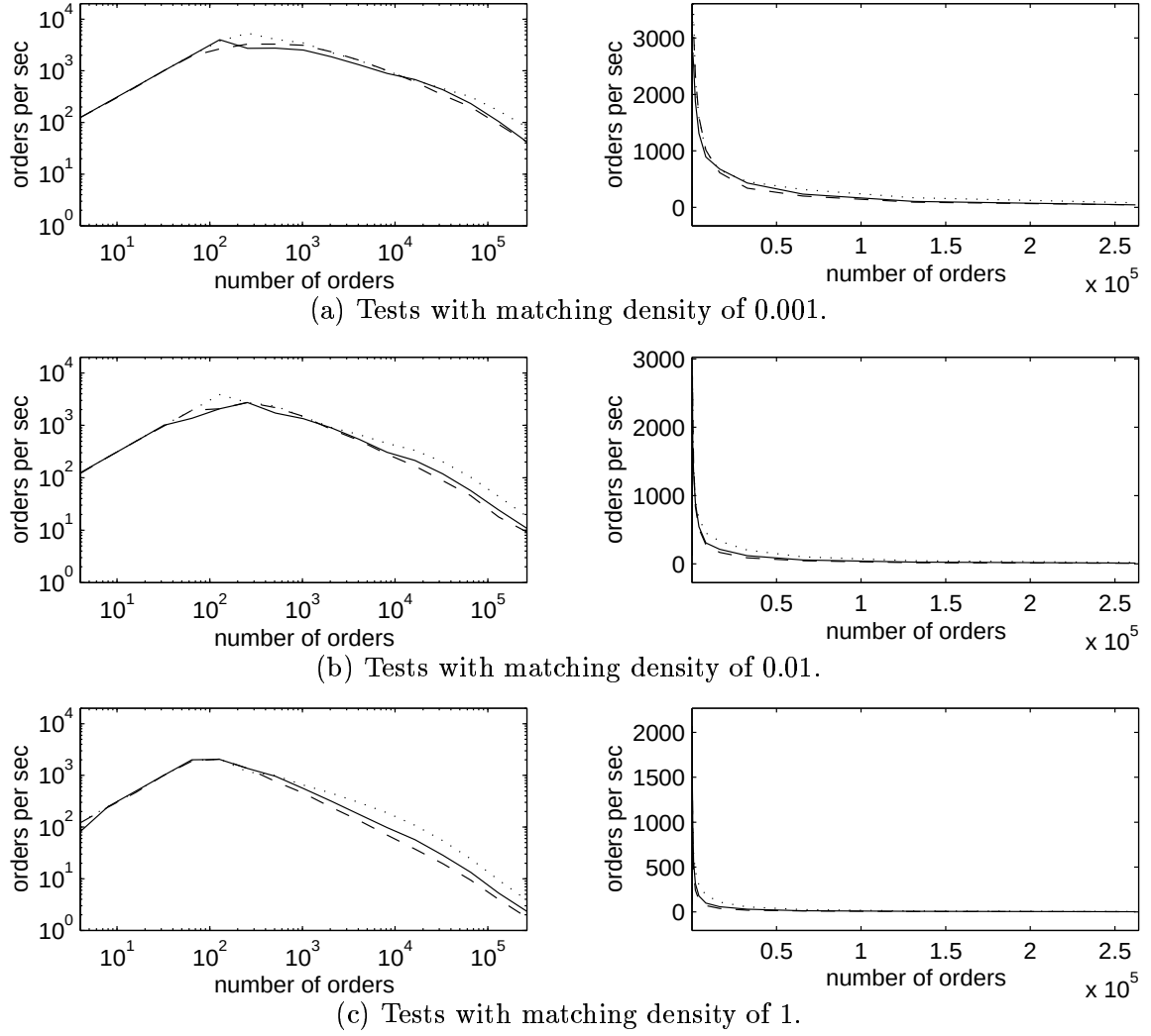
Figure 6.19: Dependency of the throughput on the number of orders. The legend is the same as in Figure 6.17.
