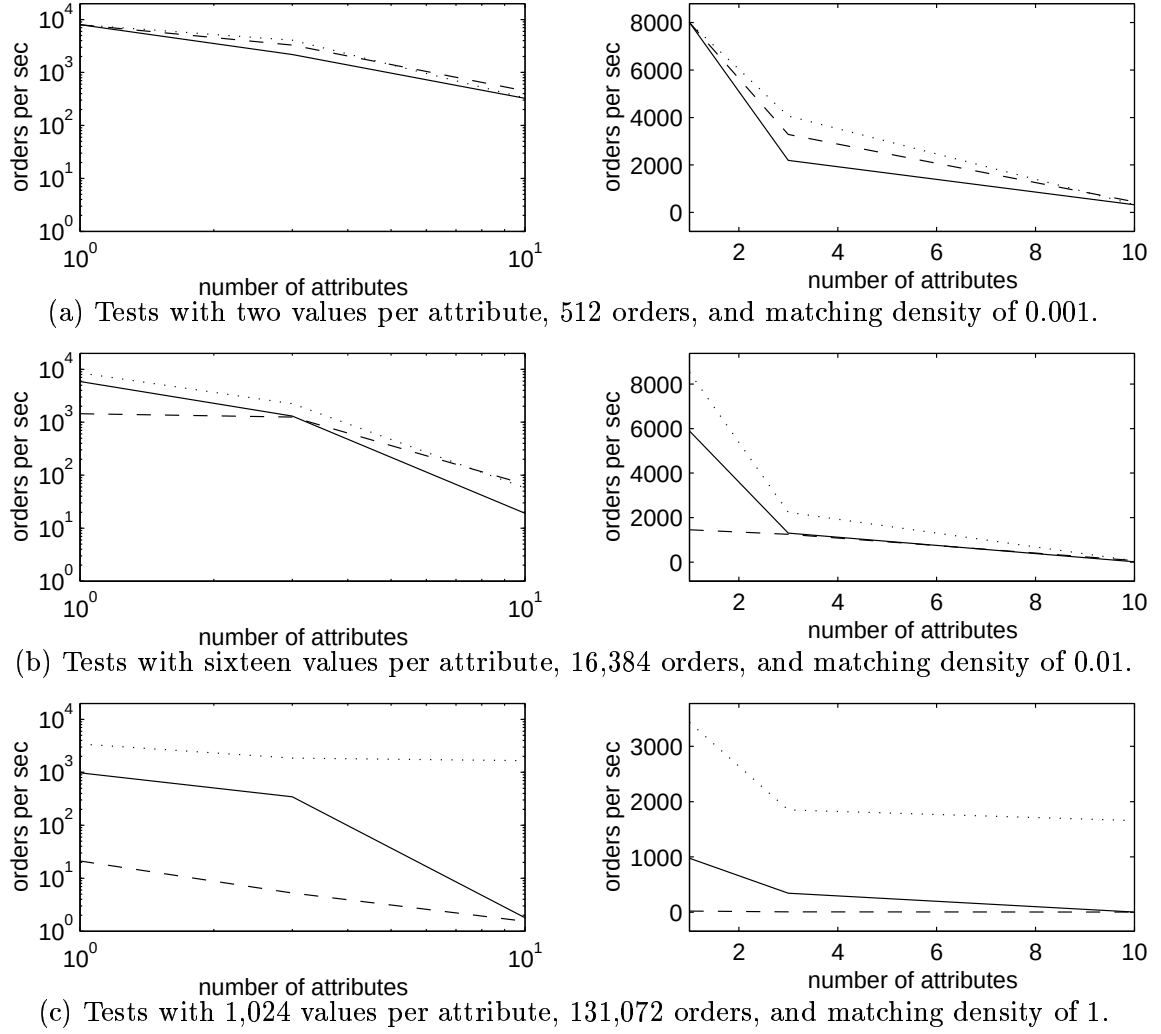
Figure 6.6: Dependency of the throughput on the number of attributes. The legend is the same as in Figure 6.1.
