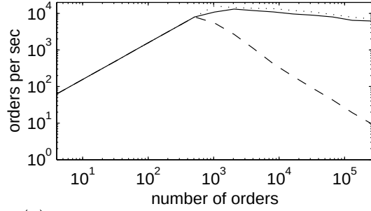
(a) Tests with one attribute, two values per attribute, and matching density of 0.001.
