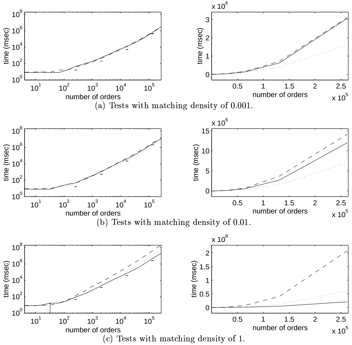
Figure 6.17: Dependency of the total matching time on the number of orders. We give the results for the best-first search (solid lines), depth-first search that identifies all matches (dashed lines), and depth-first search with a limit on the number of matches (dotted lines). The graphs on the left are in logarithmic scale, whereas the graphs on the right are in linear scale.
