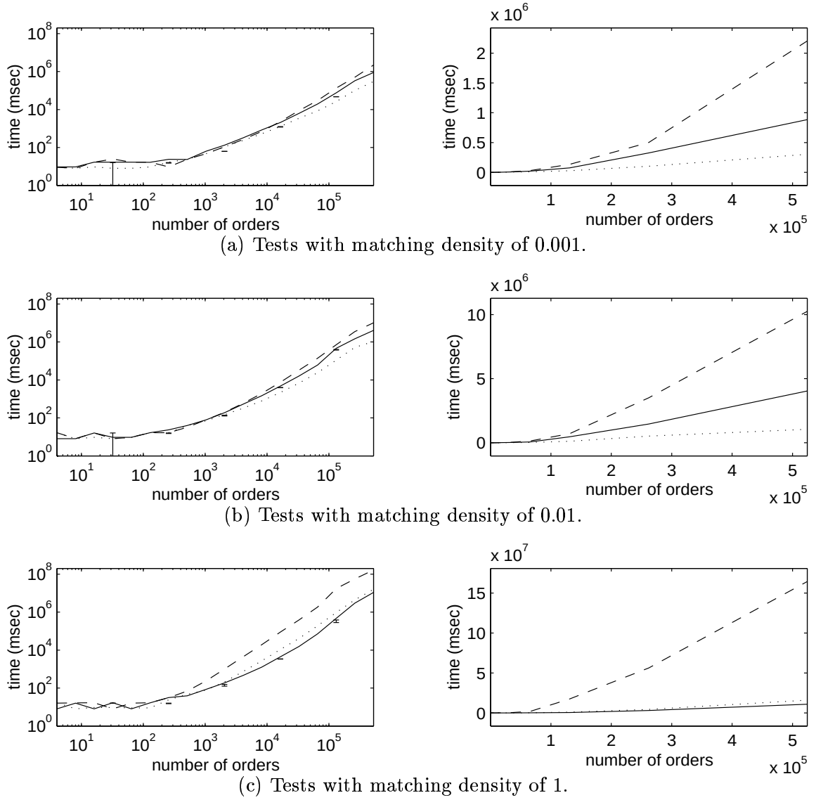
Figure 6.25: Dependency of the total matching time on the number of orders. We give the results for the best-first search (solid lines), depth-first search that identifies all matches (dashed lines), and depth-first search with a limit on the number of matches (dotted lines). The graphs on the left are in logarithmic scale, whereas the graphs on the right are in linear scale.
