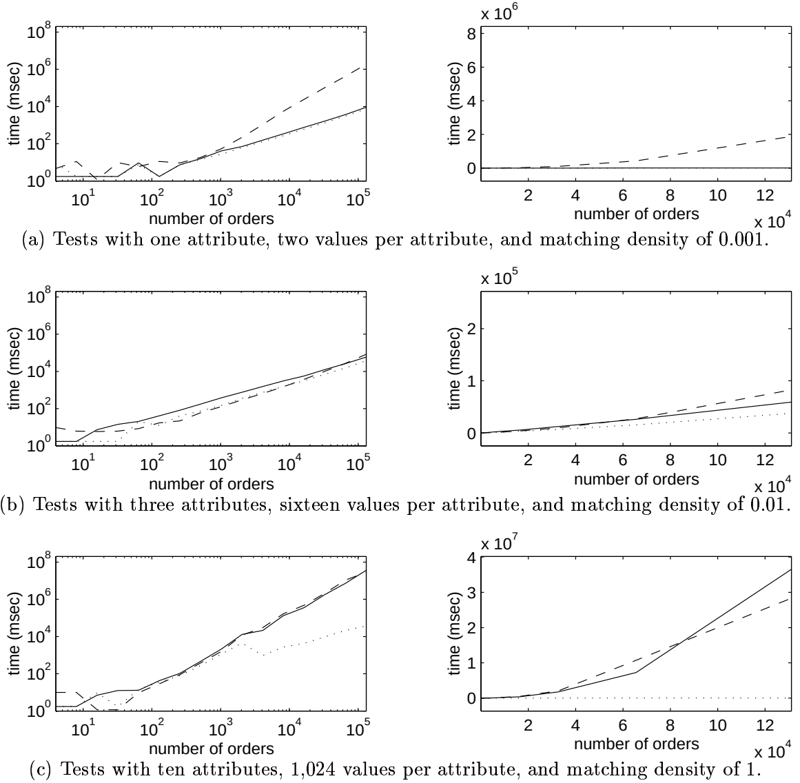
Figure 6.2: Dependency of the response time on the number of orders. The legend is the same as in Figure 6.1.
