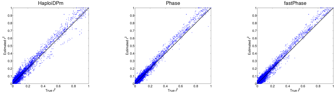
Figure 9: True ( x -axis) and estimated ( y -axis) r^2 values for each pair of loci in HapMap ENm010 region of length 254.
