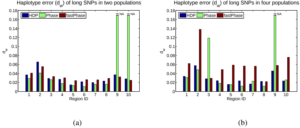
Figure 7: Performance on the full sequences of the selected ten ENCODE regions. (a) Under the two-population scenario. (b) Under the four-population scenario. For cases of which the computation did not finish within a tolerable duration (i.e., 800 hours), we cap the bar with a “ \approx ” to indicate that the results are not available (NA).
