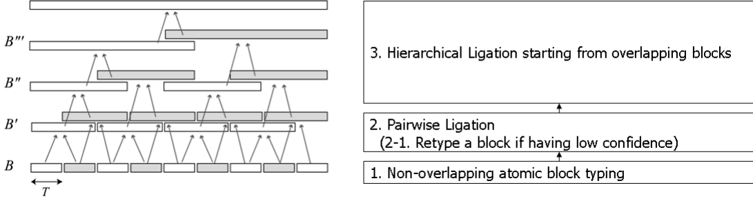
Figure 11: A hierarchical partition-ligation scheme used in Haploi .
