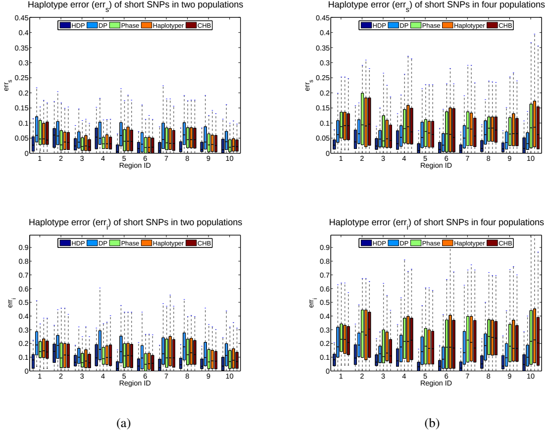
Figure 6: A comparison of haplotyping accuracies of all 7-SNP segments from 10 ENCODE regions. (a) Box-plots of error rates when data only from the CEPH and Yoruba population are used. (b) Error rates under the four-population scenario. The top row shows the summary statistics of err_s , and the bottom row shows that of err_i .
