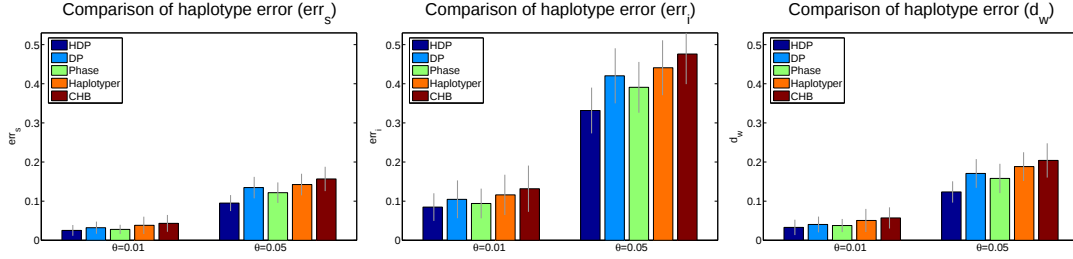
Figure 2: Performance on simulated datasets. Two kinds of datasets with different mutation rates \theta were tested. Each dataset includes 100 individuals from 5 groups (20 from each). The sequence length was fixed to 10. The performance of each algorithm is represented in terms of err_s , err_i and d_w . Each bar represents the average error rate across 50 different datasets where the standard deviation is shown as a vertical line.
