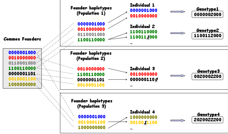
Figure 1: The haplotype-genotype generative process under HDPM, illustrated by an example concerning three populations. At the first level, all haplotype founders from different populations are drawn from a common pool via a Pólya urn scheme, which leads to the following effects: 1) the same founder can be drawn by either multiple populations (e.g., the red founder in population 1 and 2, and the blue one in population 1 and 3), or only a single population (e.g., the grey founder in population 1); 2) shared founders can have different frequencies of being inherited. Then at the second level, individual haplotypes were drawn from a population-specific founder pool also via a Pólya urn scheme, but this time through an inheritance models P_h(\cdot|a_k) that allows mutations with respect to the founders, as indicated by the underscores at the mutated loci in the individual haplotypes. Finally, the genotype observations are related to the haplotype pairs of every individual via a noisy channel P_g(\cdot|\cdot) .
