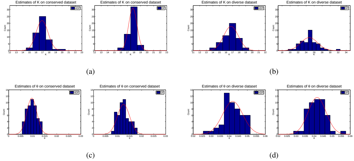
Figure 4: Top row: Histograms of the number of recovered ancestors, K , across the 50 conserved data sets (panel (a)), and across the 50 diverse data sets (panel (b)). Bottom row: Histograms of the estimated mutation rates over the 50 conserved data sets (panel (c)), and over the 50 diverse data sets (panel (d)). The left graph in each panel shows the result from HDP, and right one shows that from DP.
