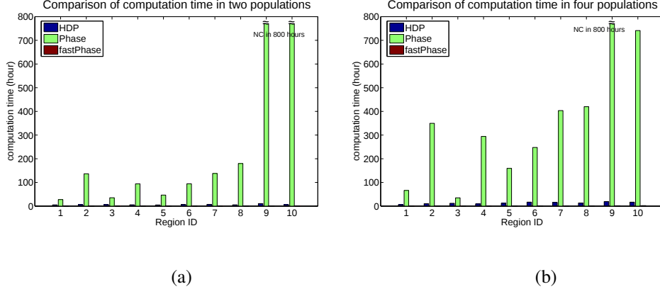
Figure 8: Time complexity on the full sequences of the selected ENCODE regions. (a) Under the two-population scenario. (b) Under the four-population scenario. We cap the bars corresponding to not-completed (NC) cases with a “ \approx ”.
