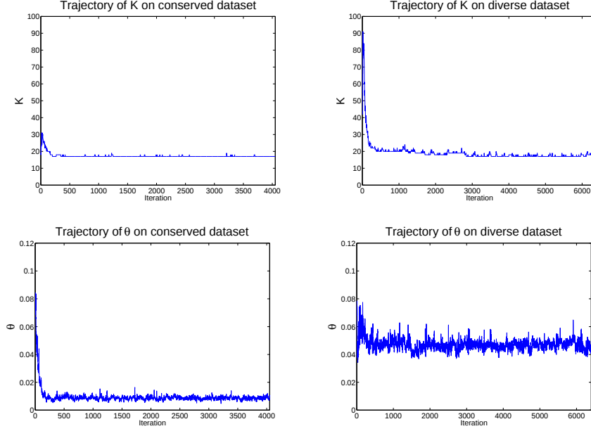
Figure 3: Trajectories of K and \theta along the iterations of HDP inference from one among the simulated datasets. The left panels show the result on conserved dataset, and the right, on diverse dataset.
