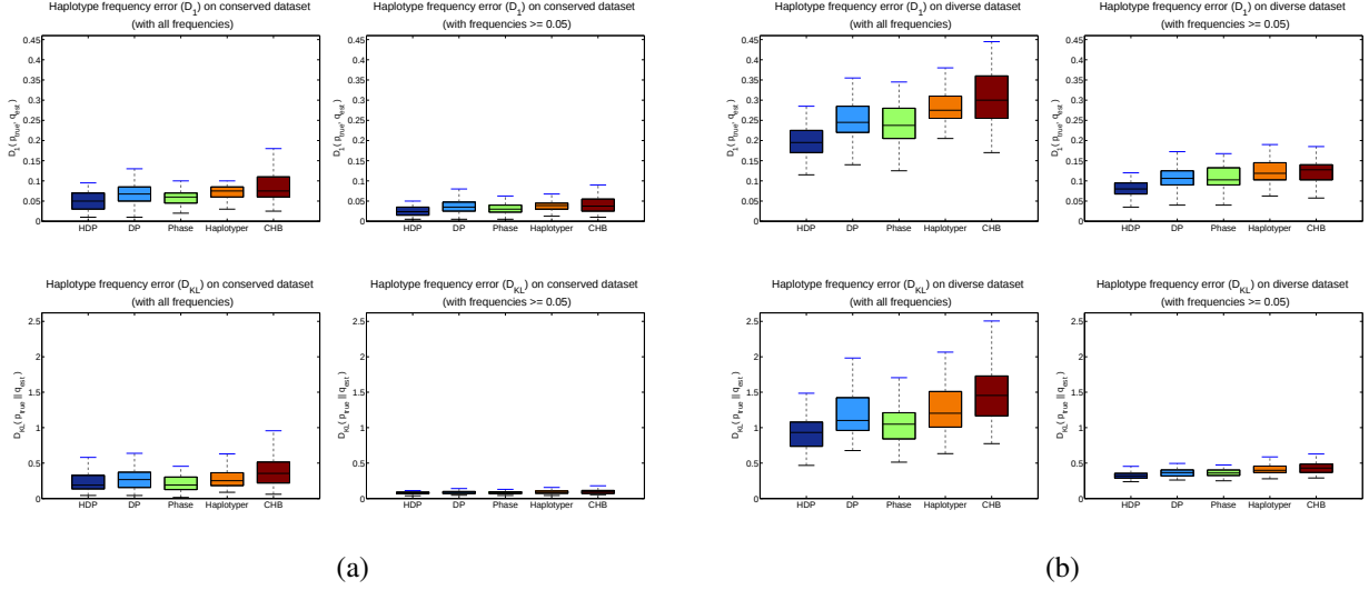
Figure 5: A comparison of the accuracies of haplotype frequencies estimated by five algorithms. (a) Box-plots of D_1 's (top) and D_{KL} 's (bottom) estimated from the conserved data sets. Left column shows measurements on all haplotypes, right column shows measurements on only the frequent haplotypes. (b) Same measurements on the diverse datasets.
