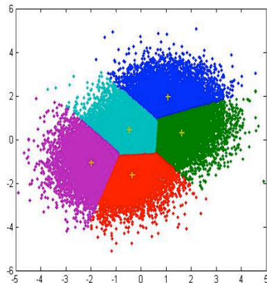
K-means
