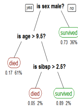
Decision trees
