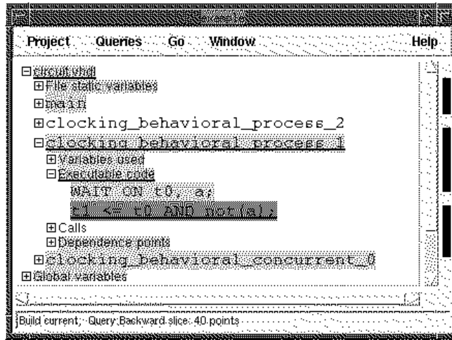
Figure 10: Backward slice on t1 \leq t0 \text{ AND } \text{not}(a);
