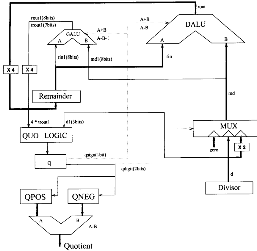
Figure 1. The division circuit.
