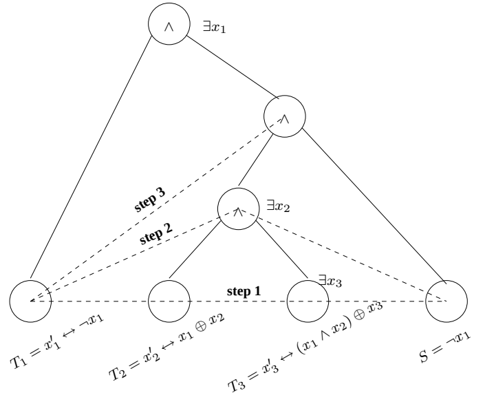
Figure 2: Dynamic VarScore algorithm in action. The dotted lines represent the BDDs in the set F at different iterations of the VARSOREBASICSTEP.
