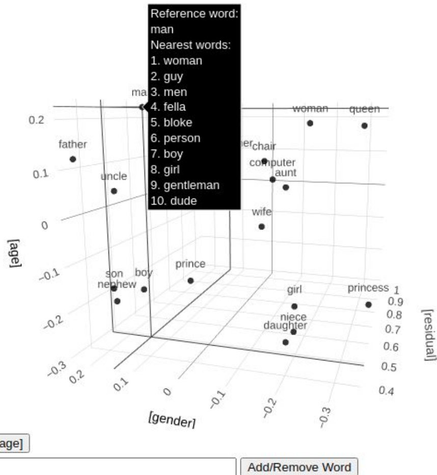
Word vector projection
