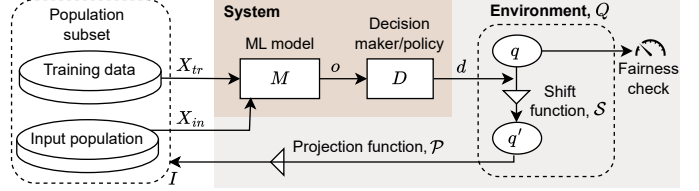
Fig. 3: Feedback loop model of ML-enabled system
