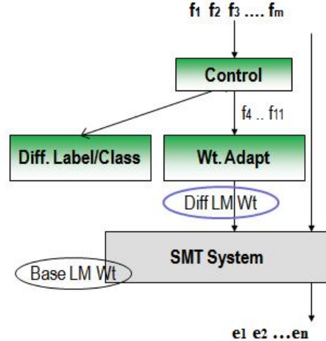
Figure 1: The SMT pipeline with difficulty classifier and LM weight adaptation
